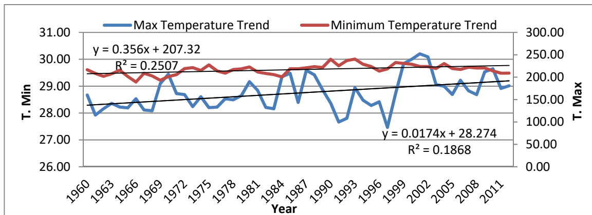
Figure 5. Annual minimum and maximum temperature trends.
