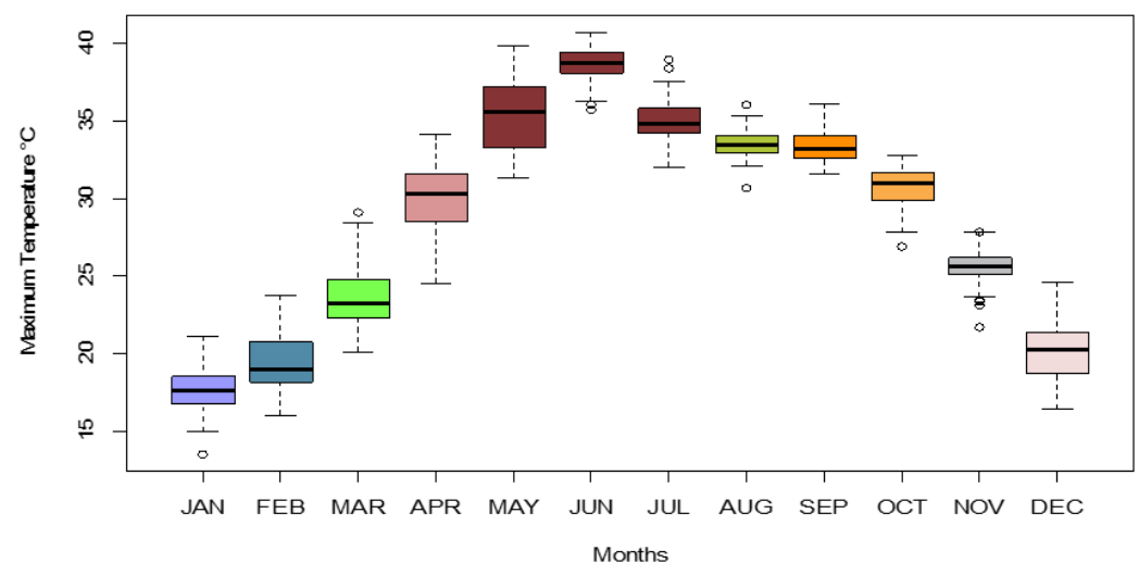
Figure 7. Monthly Tmax readings of Islamabad city.
