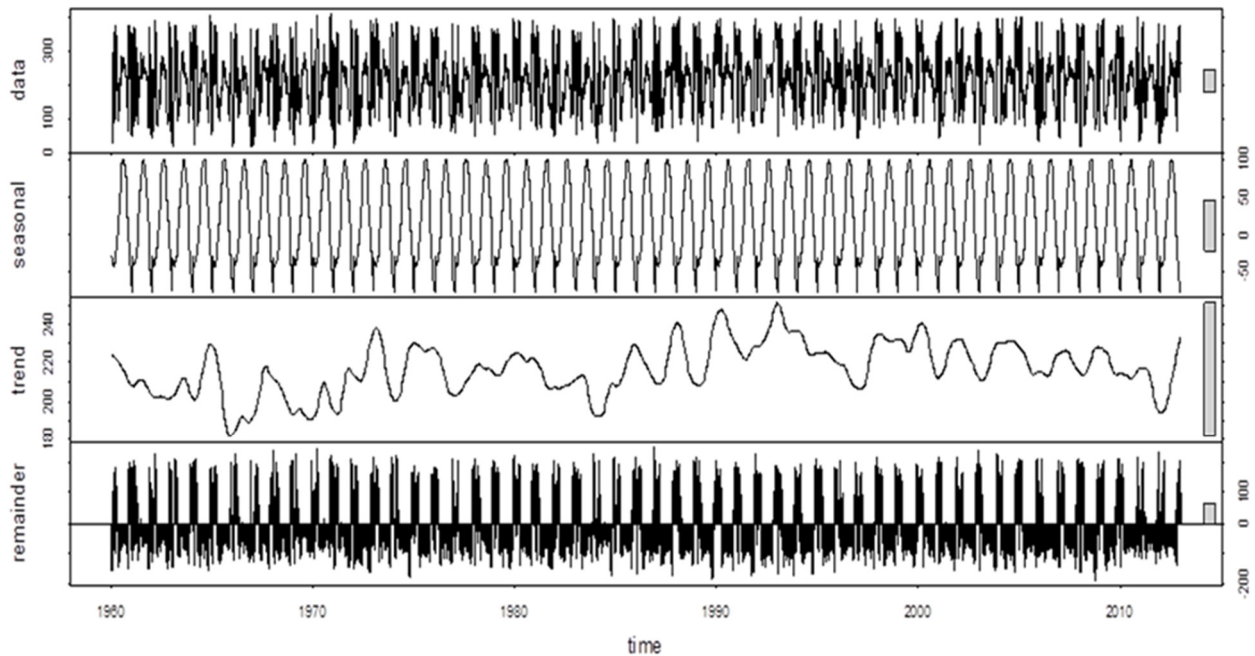
Figure 4. Minimum Temperature (Tmax).
