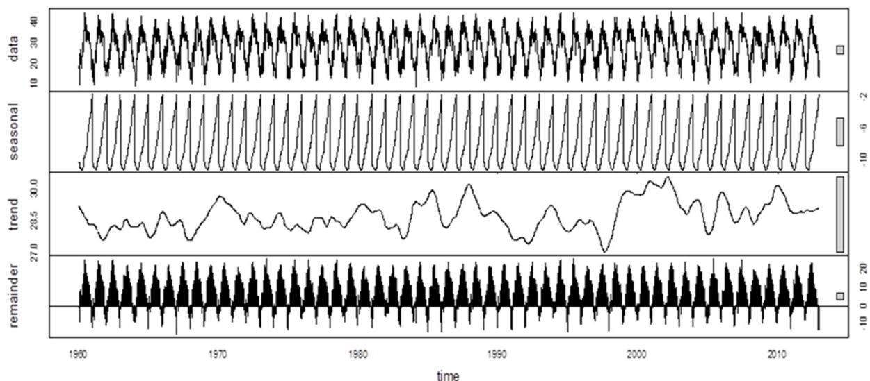
Figure 3. Maximum Temperature ( T_{max} ).
