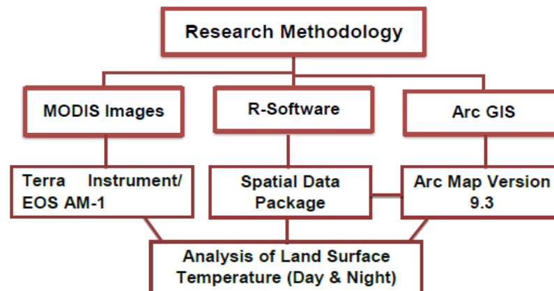
Figure 2. Flow Chart of Research Methodology.
