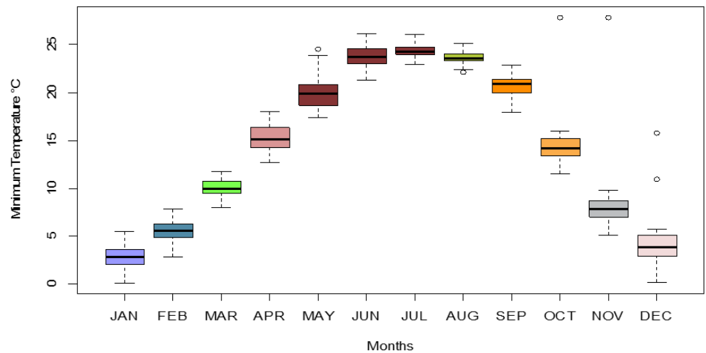
Figure 6. Monthly Tmin readings of Islamabad city.
