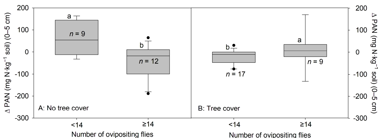
Figure 13. Soil \Delta PAN (change in plant-available N, 0–5 cm depth) when ovipositing flies per chamber were <14 or \geq 14 . (A) Manure pats that were under no cover, and (B) manure pats that were under tree cover. Negative numbers indicate a loss in PAN and different lowercase letters indicate a significant difference ( p < 0.05 ).
