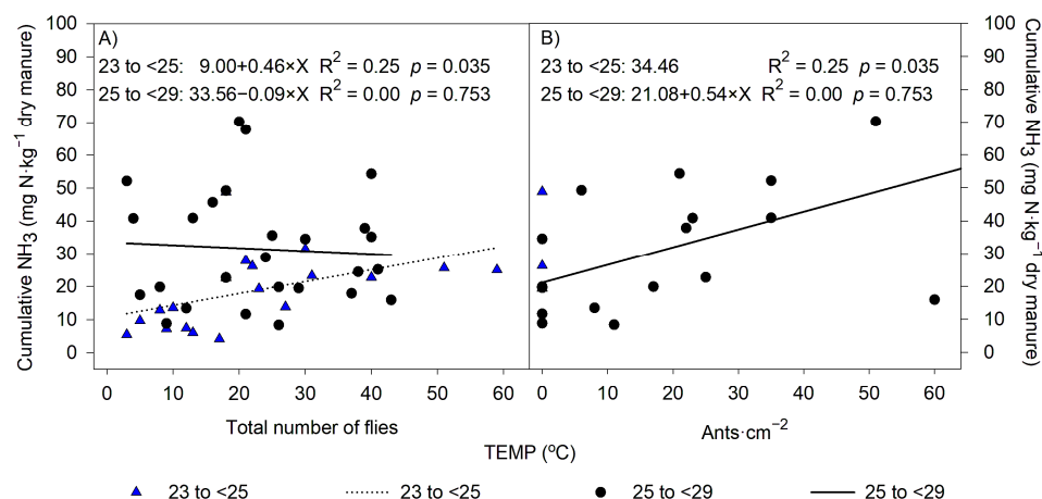
Figure 5. (A) Cumulative NH 3 emitted during the 16-day sampling period vs. the total number of flies that oviposited or emerged from manure pat, under two ranges of daily average temperature (23 to <25 °C and ≥25 to <29 °C). (B) Cumulative NH 3 emitted during the 16-day sampling period vs. the total number of ants per square centimeter that were recorded per manure pat, under two ranges of daily average temperature (23 to <25 °C and ≥25 to <29 °C).
