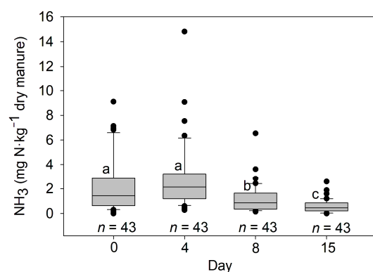
Figure 6. NH 3 emissions measured 0, 4, 8, and 15 days after manure deposition. Different letters indicate a significant difference ( p < 0.05 ).
