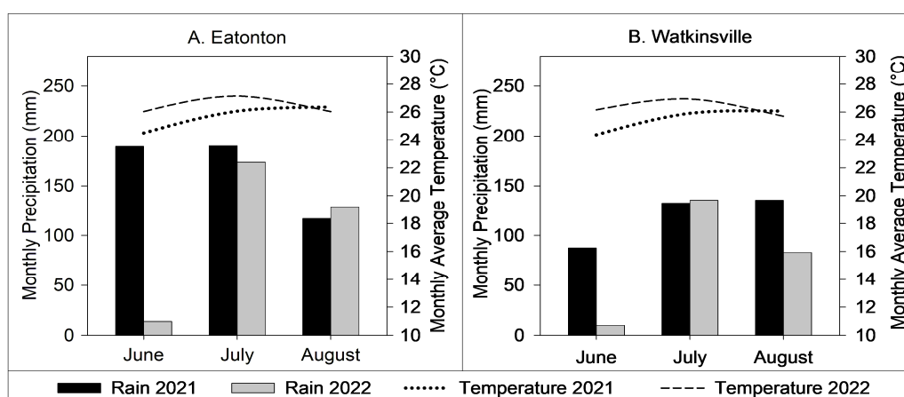
Figure 1. Monthly precipitation and average monthly temperature for 2021 and 2022 for (A) Eatonton and (B) Watkinsville.
