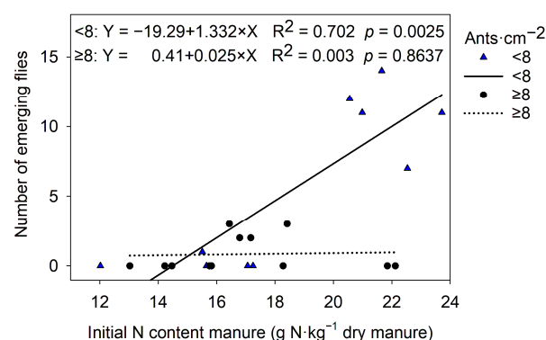
Figure 3. The number of flies emerging from manure (day 15/16) vs. initial nitrogen (day 0) content in manure under two ranges of ant count per square centimeter.
