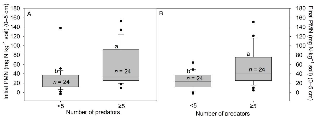
Figure 15. (A) Initial soil PMN and (B) final soil PMN (0–5 cm depth) when predators per chamber were <5 or ≥5. Different lowercase letters indicate a significant difference ( p < 0.05 ).
