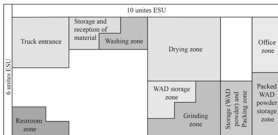
Figure 10. Theoretical plant layout.
