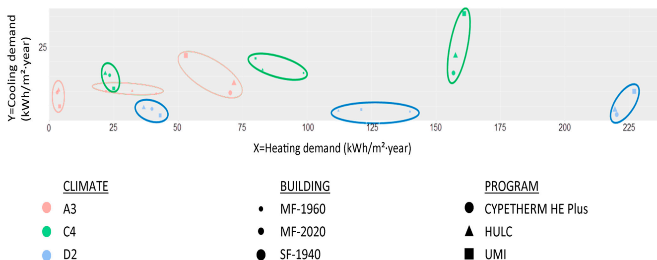
Figure 7. Graphical representation of the heating and cooling demand results from the three models in the three climates and using the three programs.
