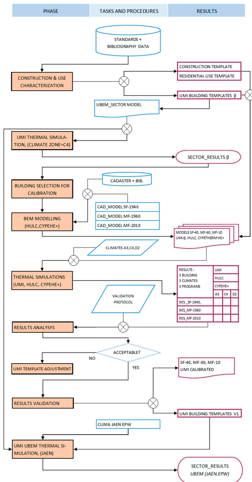
Figure 3. Workflow for the validation of the GIS-UBEM.
