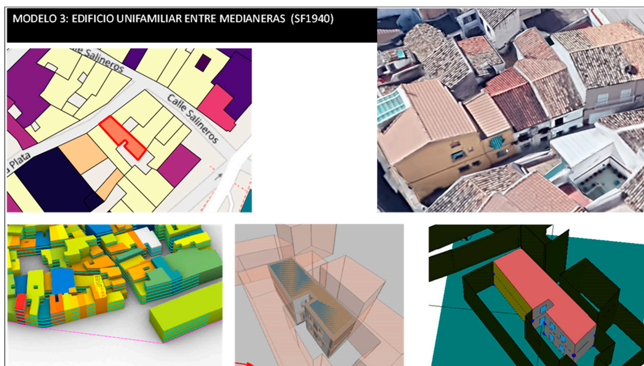
MODEL 3: SEMIDETACHED SINGLE-FAMILY HOUSE (SF1940).
