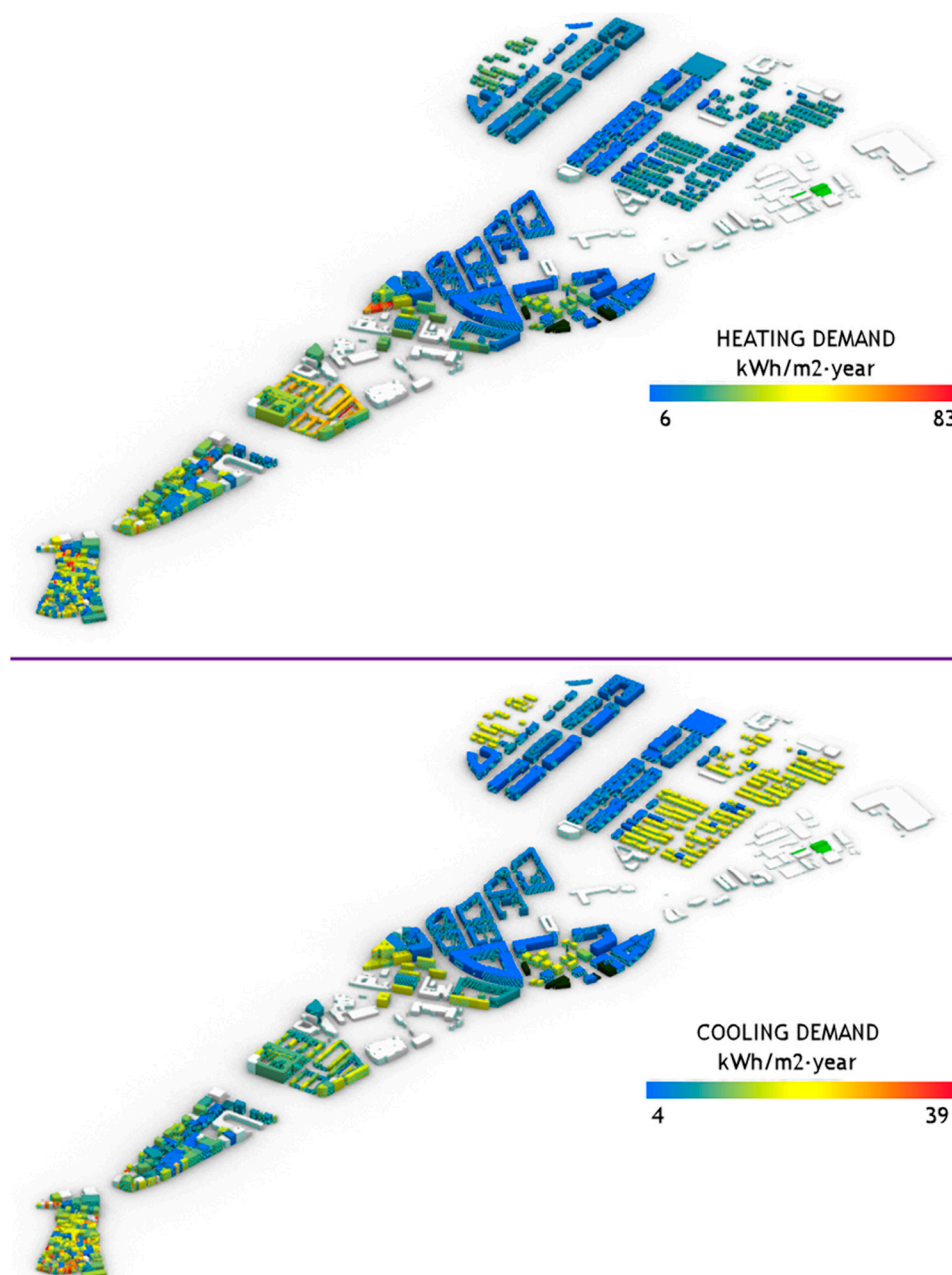
Figure 8. False color representation of heating and cooling demands normalized per square meter in the Jaén sector. Results from the GIS-UBEM obtained with the UMI.
