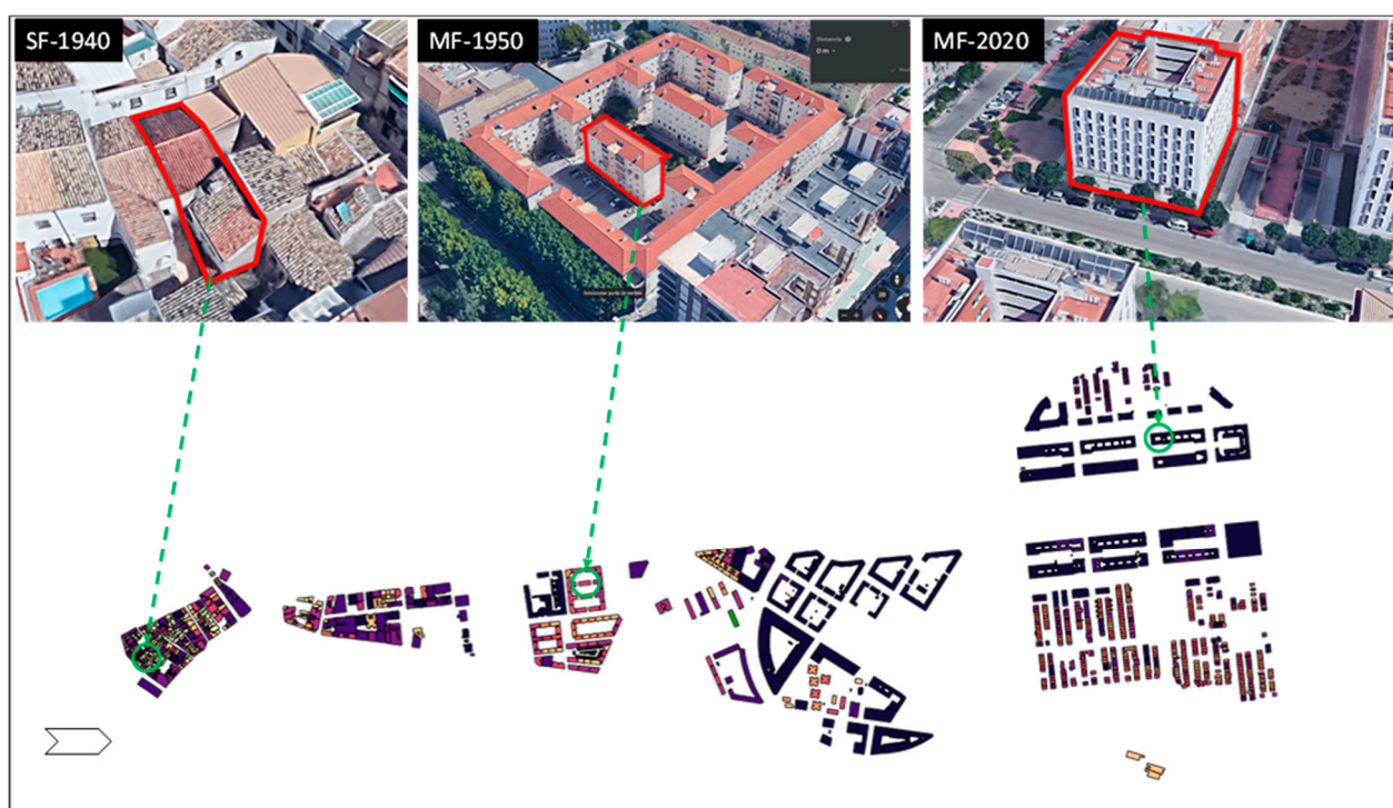
Figure 6. Selected benchmark buildings. Aerial view and location within the case study area in Jaén. Color ramp represents building's heating demand per m^2 .
