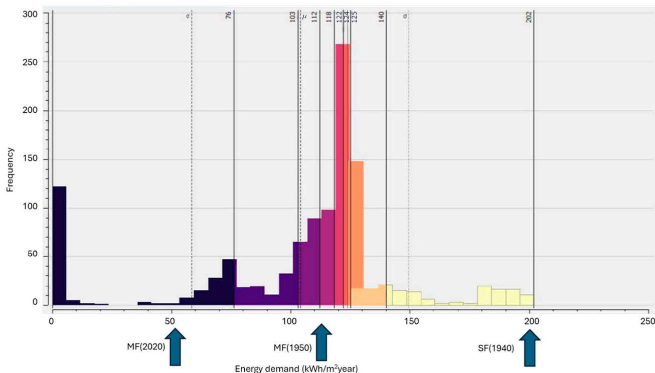
Figure 5. Histogram of preliminary calculation results of consumption for the buildings in the study sample. Colours represent deciles of the building population.
