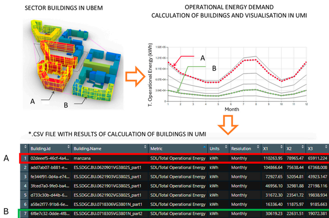
Figure 4. Sample output of results of buildings A and B from a UBEM model in UMI. Exploration of consumption results by different uses on a monthly basis. The results were imported in CSV format for processing and statistical analysis in R-Studio 2022.02.0. Note: *.CSV is used to represent
