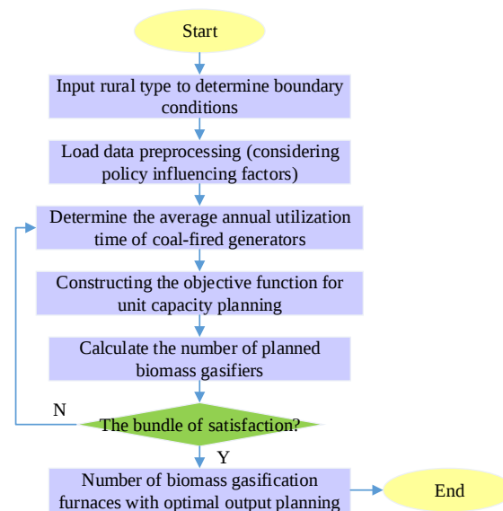
Figure 3. Capacity optimization of biomass-coal coupling units.
