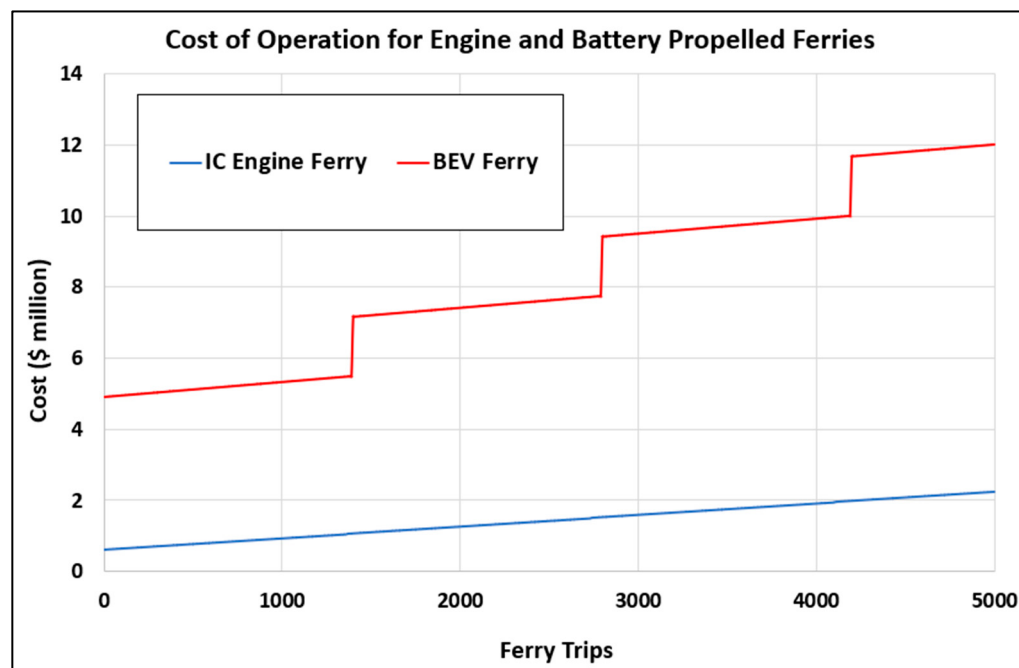
Figure 13. Cost of operation for BEV and IC engine configurations of the Mackinac Island ferry.
