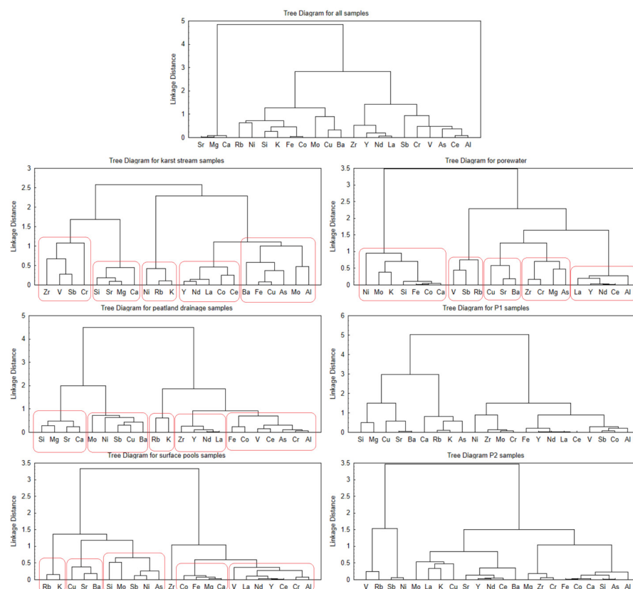
Figure 7. Cluster analysis results for each separate water type. Cluster groups are marked for the main water types (karst stream, drainage stream, surface pool, and pore water). The figure also includes a cluster analysis of all the samples and the individual locations of the pore water. Included in the analysis are measured elemental concentrations.
