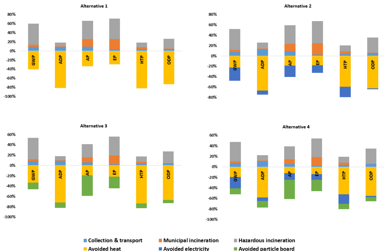
Figure 3. Contribution of the process to the various environmental impacts for different alternatives.
