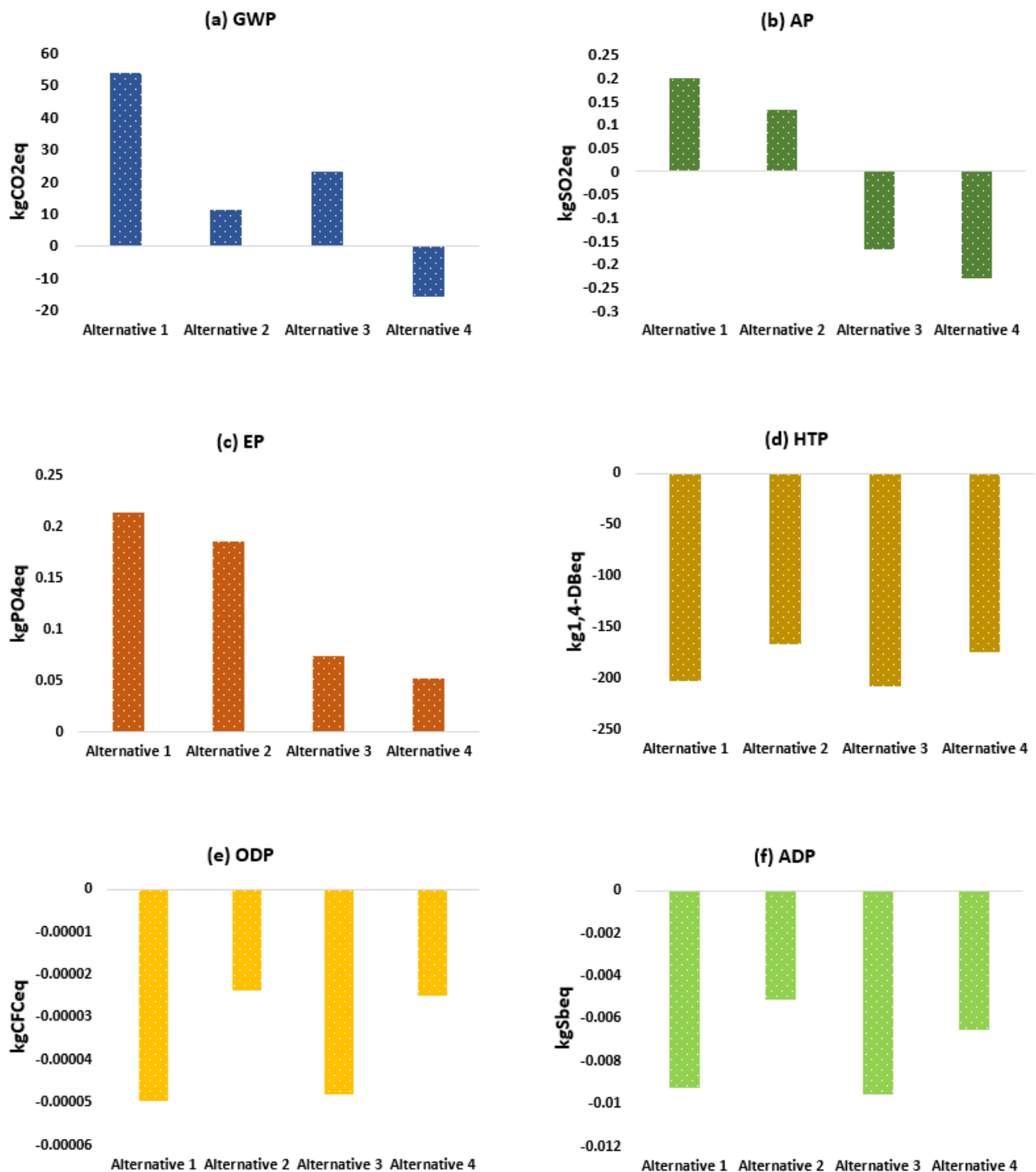
Figure 2. Environmental impacts of the four alternatives per functional unit: (a) global warming potential (GWP), (b) acidification potential (AP), (c) eutrophication potential (EP), (d) human toxicity potential (HTP), (e) ozone depleting potential (ODP), and (f) abiotic depletion potential (ADP).
