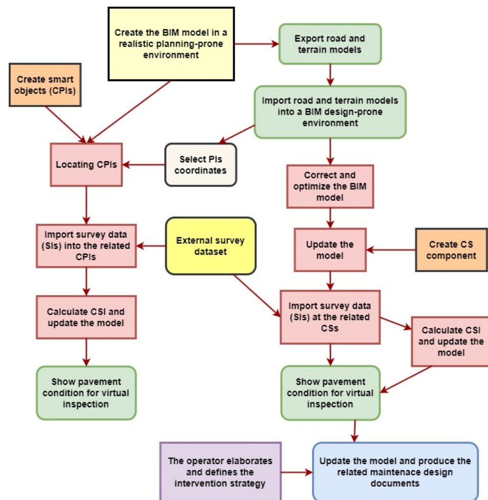
Figure 1. Flowchart of the proposed operative framework (CPI: Condition Point of Interest; PI: Point of Interest; CS: Condition Subassembly; SI: State Indicator; CSI: Critical State Index).
