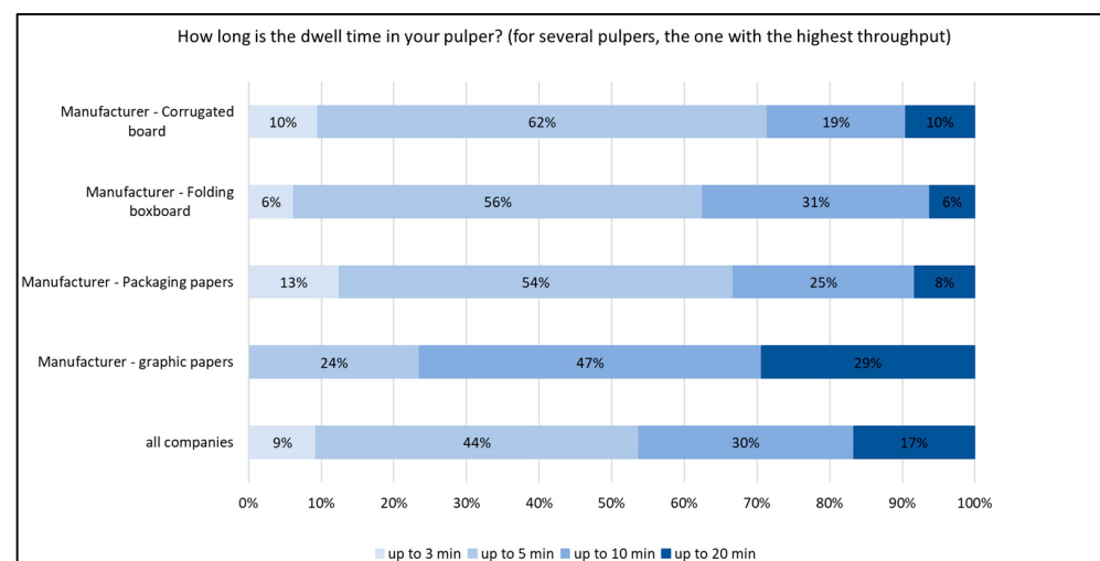
Figure 17. Dwell time in the pulper in relation to the produced paper (manufacturer-corrugated board n = 21 , manufacturer-folding boxboard n = 16 , manufacturer-packaging papers n = 24 , manufacturer-graphic papers n = 17 , all companies n = 54 ; one company can produce several products).
