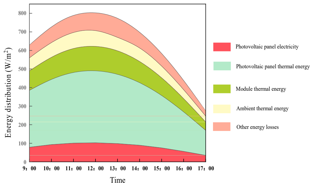
Figure 9. Energy distribution of independent PV module.
