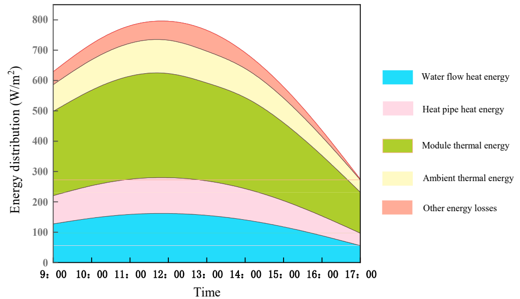
Figure 10. Energy distribution of independent heat collection modules.
