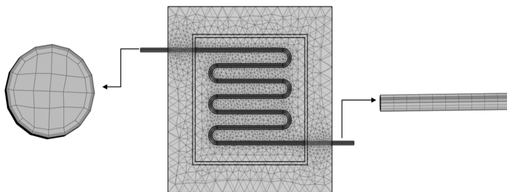
Figure 2. PIPVT cell meshing diagram.
