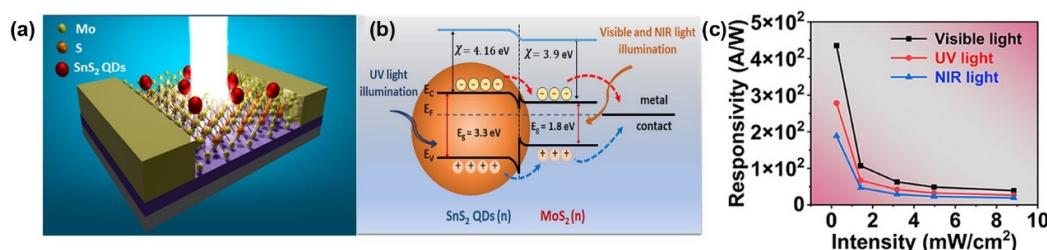
Figure 12. (a) A 3D schematic representation of \text{SnS}_2 -QDs/ \text{MoS}_2 PD. (b) Schematic illustration of band structures of \text{SnS}_2 QDs and monolayer \text{MoS}_2 . (c) R of \text{SnS}_2 -QDs/ \text{MoS}_2 PD. Reproduced with permission from ref. [174]. Copyright 2022 American Chemical Society.
