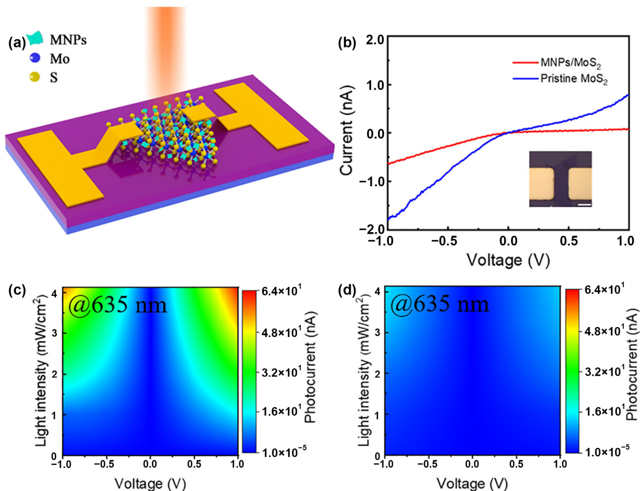
Figure 11. (a) Schematic representation of MoS 2 PD (MNPs refer to the MXene QDs with an average size of 8 nm). (b) I-V plots of pristine MoS 2 and MXene-QD/MoS 2 PD in the dark. Two-dimensional photoresponse maps of (c) MXene-QD/MoS 2 PDs and (d) pristine MoS 2 under 635 nm excitation wavelengths. Reproduced with permission from ref. [176]. Copyright 2022 American Chemical Society.
