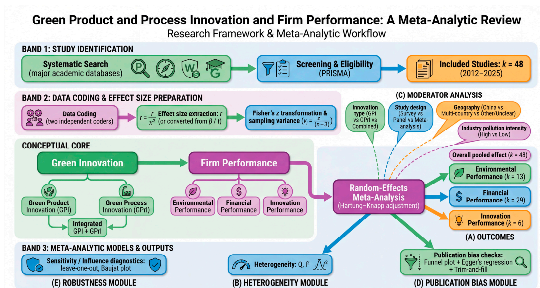
Figure 1. Research Framework.
