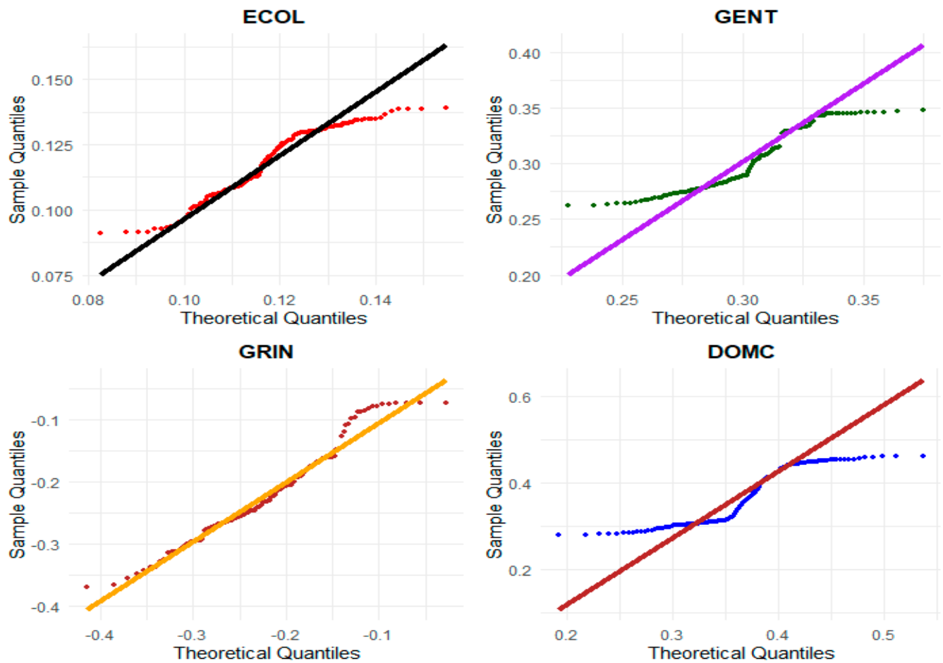
Figure 1. QQ plots.
