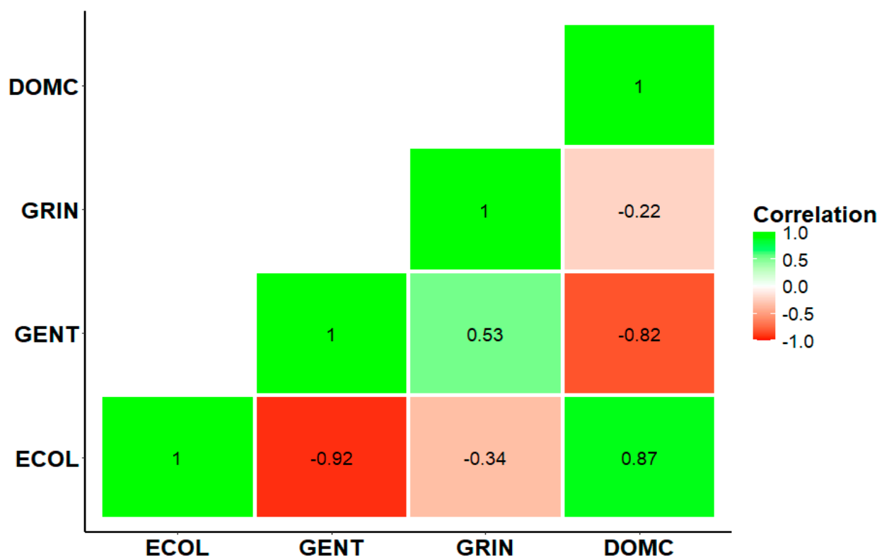
Figure 2. Correlation matrix.
