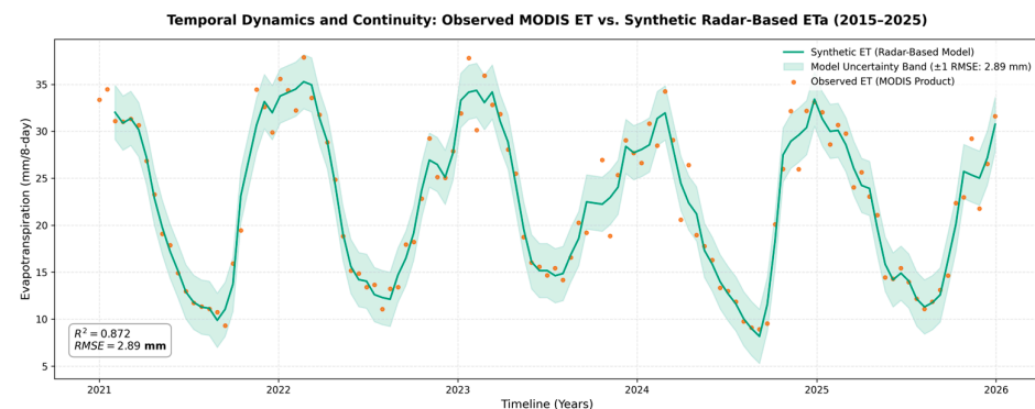
Figure 5. Temporal dynamics and validation of the synthetic radar-based actual evapotranspiration ( ET_a , continuous green line) against the observed MODIS ET product (orange scatter points) across the evaluation timeline. The plot illustrates high seasonal alignment, capturing annual agricultural peaks and water deficit troughs, confirming the model's capacity to preserve phenological integrity and maintain data continuity.
