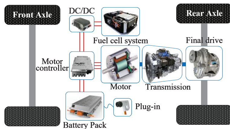
Figure 1. Powertrain architecture of the FCHECV [42].
