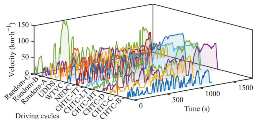
Figure 10. Test driving cycles.
