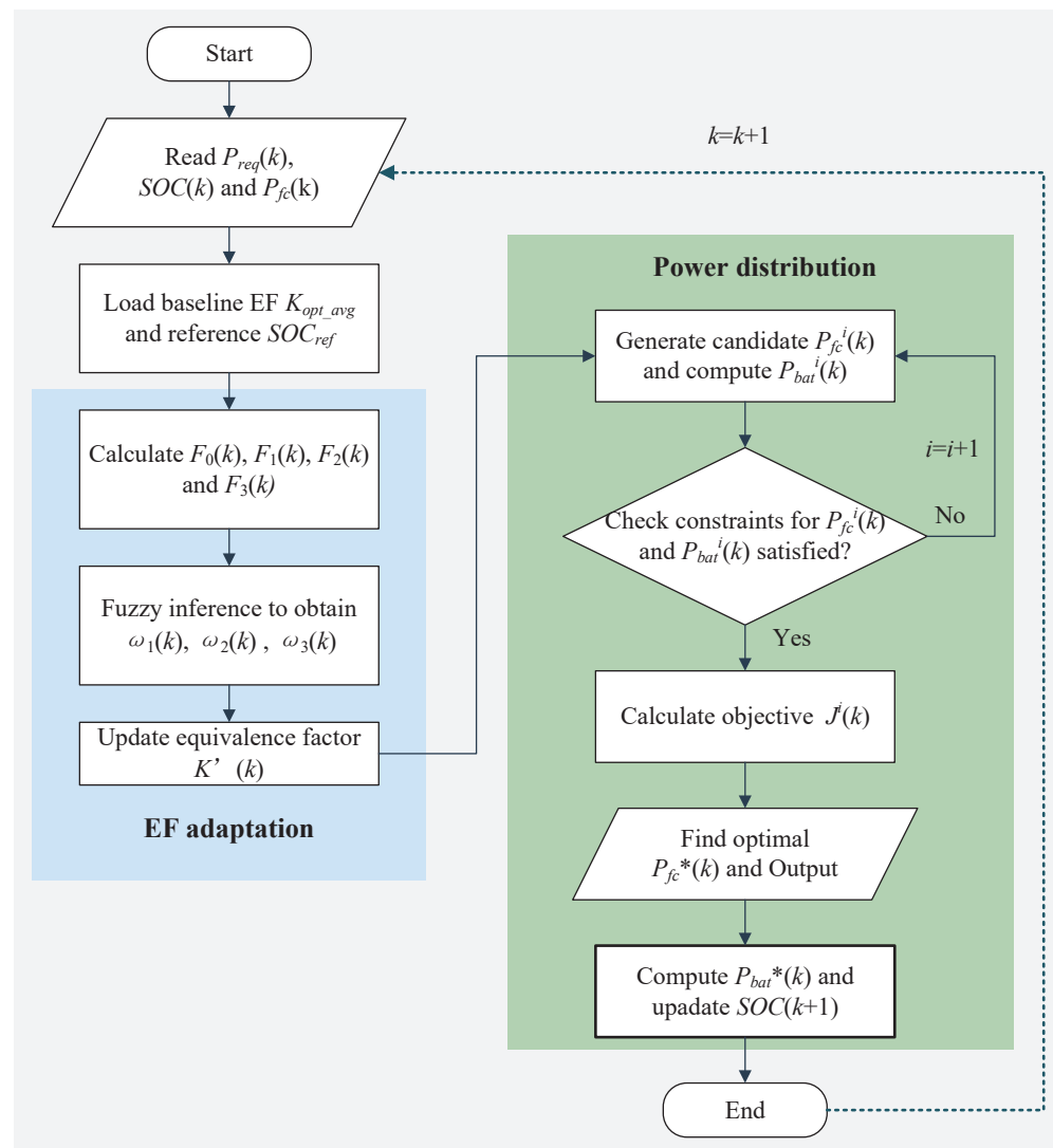
Figure 9. Flowchart of the MFCA-ECMS.
