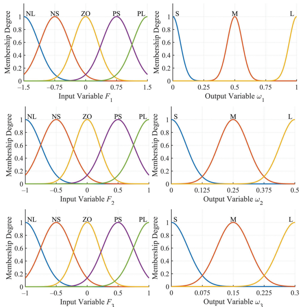
Figure 8. Membership functions for input and output variables.
