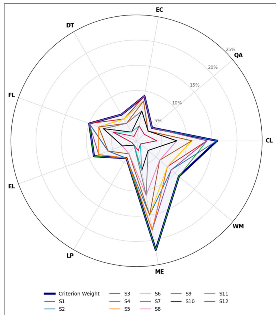
Figure 3. Criteria and suppliers comparison. Radar chart showing multiple suppliers compared across criteria.
