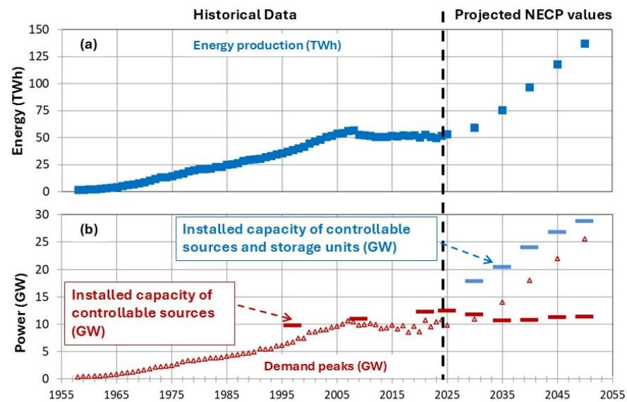
Figure 1. Historical evolution (1958–2025) of annual electricity production (a) and peak hourly demand (b) vs. installed capacity of controllable sources and storage units in the interconnected system of Greece, and projected values up to 2050, according to the NECP assumptions.
