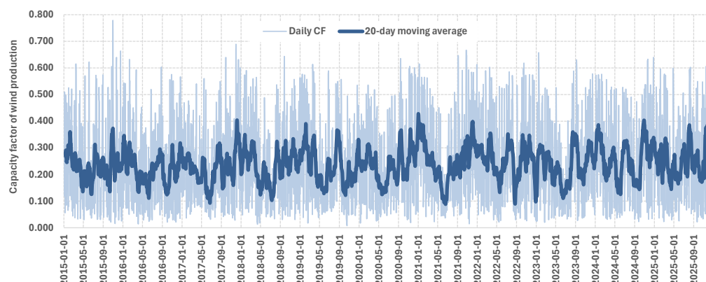
Figure 5. Capacity factor of wind power production from 2015 to 2025 across two scales (daily, 20-day moving average).
