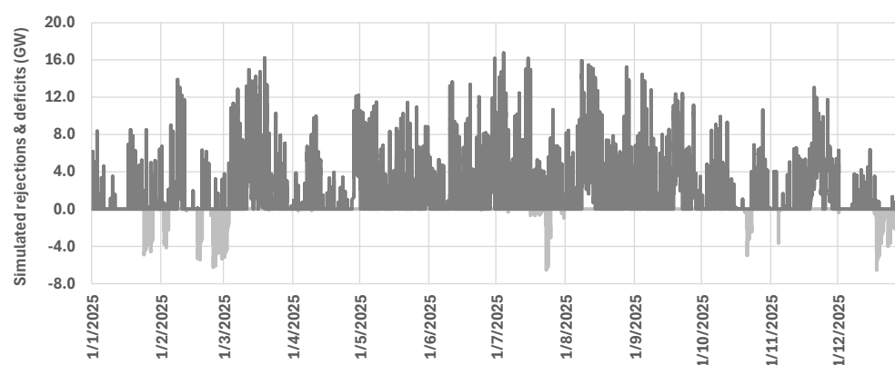
Figure 10. Simulated power rejections (dark grey, positive values) and deficits (light grey, negative values) for scenario 6 ( \lambda_{RE} = 3.0 , S_{max} = 256 GWh, and P_{max} = 5.33 GW).
