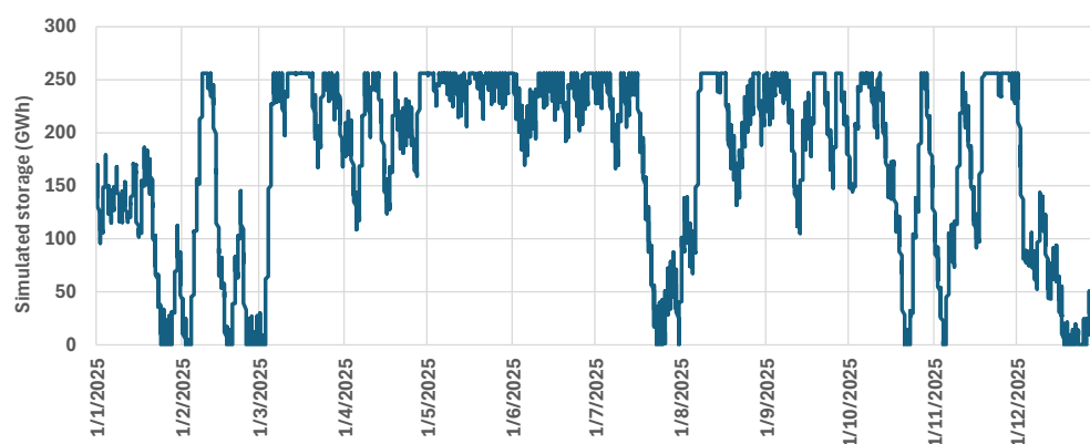
Figure 9. Simulated energy storage for scenario 6 ( \lambda_{RE} = 3.0 , S_{max} = 256 GWh, and P_{max} = 5.33 GW).
