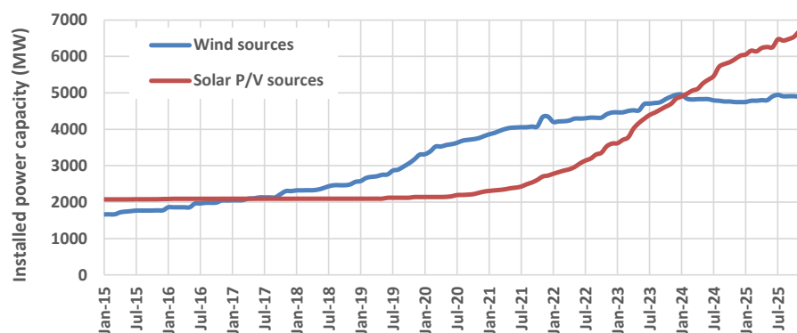
Figure 3. Monthly evolution of the installed capacity of wind and solar P/V sources during 2015–2025.
