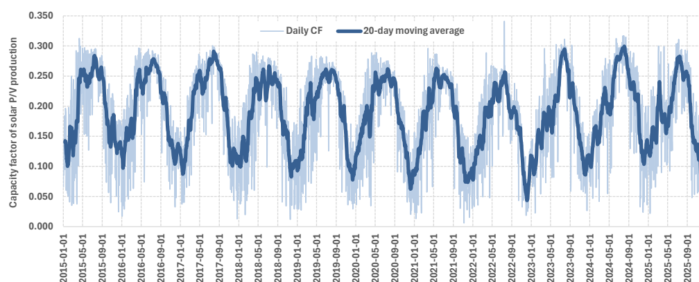
Figure 6. Capacity factor of solar P/V energy production from 2015 to 2025 across two scales (daily and 20-day moving average).
