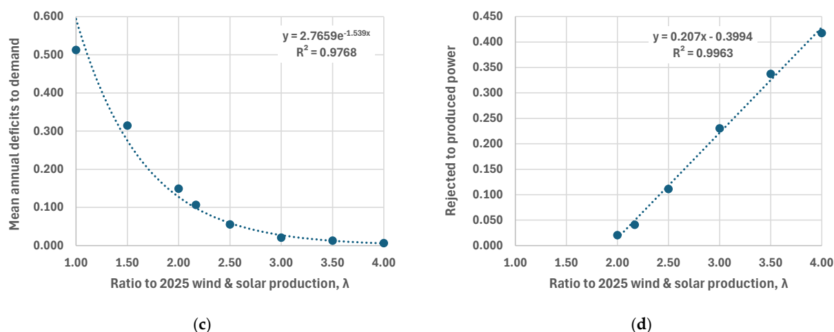
Figure 11. Scatted plots of the key quantities of interest with respect to the 2025 production from wind and solar P/V sources: (a) optimized energy storage and power capacity; (b) failure probability; (c) mean annual deficits-to-demand ratio; (d) rejected-to-produced energy by all renewables (wind, solar, and hydro).
