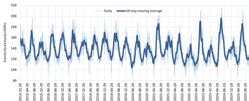
Figure 7. Electricity demand from 2015 to 2025 across two scales (daily and 20-day moving average).
