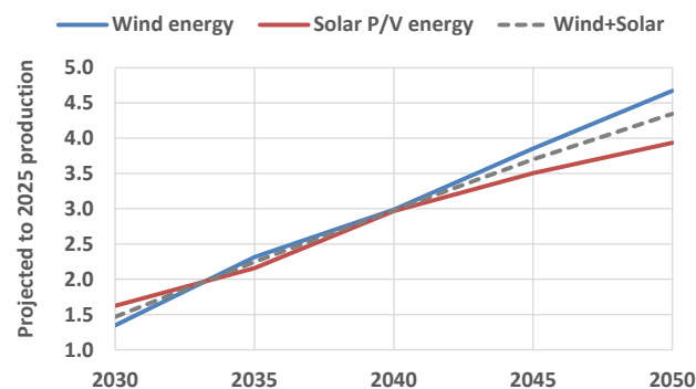
Figure 8. NECP's projections of wind and solar P/V production, divided by the 2025 values.
