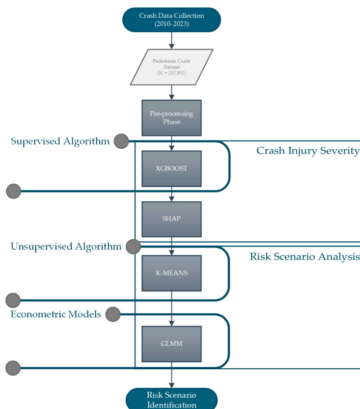
Figure 1. Flow chart of the Risk Scenario Identification Methodology.
