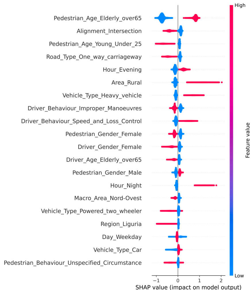
Figure 4. Graphical results of SHAP analysis.
