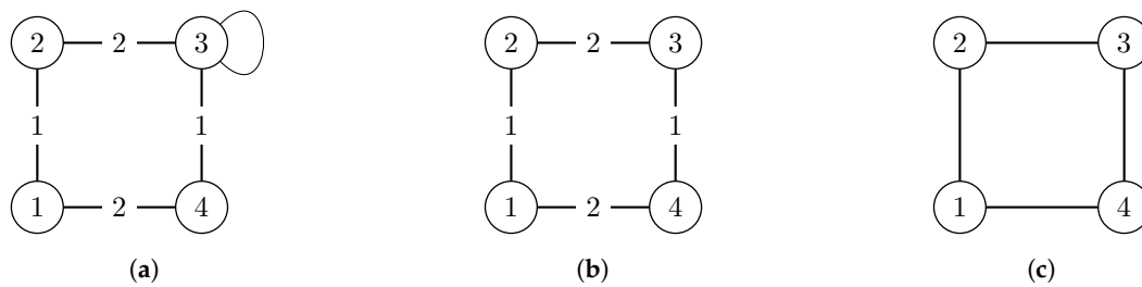
Figure 1. Example of a two-step simplification of the graph G_{w+1} (left) which is asymmetric. G_w in the middle is still weighted but has a non-trivial automorphism group and G (right) is simple with a more complex automorphism group. Each automorphism group of the more complex graph(s) is a subgroup of the simpler graph(s): Aut(G_{w+1}) \leq Aut(G_w) \leq Aut(G_w) . This example shows how simplification of graphs by removing weights and/or loops can lead to additional symmetries. (a) The weighted graph G_{w+1} which also has a loop at node 3. It has the trivial automorphism group Aut(G_{w+1}) = \{1\} . (b) A simplified version G_w of the graph G_{w+1} with the following symmetries: Aut(G_w) = \{1, (12)(34), (23)(14), (13)(24)\} . (c) The simple graph G which has the automorphism group Aut(G) = Aut(G_w) \cup \{(13), (24), (1234), (1432)\} .
