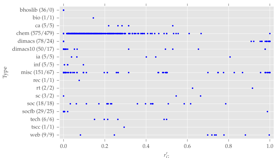
Figure 5. The normalized redundancy distributions per class. The classes are (as named on networkrepository.com ): bhoslib (“BHOSLIB”), bio (“Biological Networks”), ca (“Collaboration Networks”), chem (“Cheminformatics”), dimacs (“DIMACS”), dimacs10 (“DIMACS10”), ia (“Interaction Networks”), inf (“Infrastructure Networks”), misc (“Miscellaneous Networks”), rec (“Recommendation Networks”), rt (“Retweet Networks”), sc (“Scientific Computing”), soc (“Social Networks”), socfb (“Facebook Networks”), tech (“Technological Networks”), tscc (“Temporal Reachability Networks”), web (“Web Graphs”). After each class name, the tuple (“number of class members”, “number of symmetric class members”) is given. For this plot, duplicates from different classes were not removed to prevent a bias within classes. 975 networks are spread over the 17 classes. Details on the six largest classes are given in the text. The distributions of normalized redundancy per class differ strongly and with an exception of bhoslib, each class contains a large amount of symmetric graphs.
