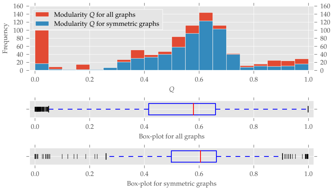
Figure 3. The histogram and box-plots for the modularity Q as a measure of cluster structure. All bins have an equal width of 0.05. Again, many graphs with partitions having a certain modularity value Q are found to be symmetric. Only graphs with a very low modularity seem to be substantially less symmetric, which is discussed in the text. There is no concise definition for which values of Q a partition of a graph is good, because this depends on the graph’s size. For smaller graphs, values greater than 0.3 are fine, for large graphs, values greater 0.9 are not unusual.
