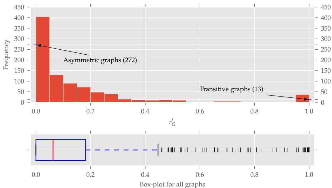
Figure 4. The histogram and box-plot for the normalized redundancy r'_G for all 902 graphs. In total, there are 272 asymmetric and 13 completely symmetric (transitive) graphs. Most of the graphs have a quite low normalized redundancy, nevertheless about 70% of the analyzed data contain symmetries. The bin width is 0.05. The right skew of the distribution is underlined by the often-true relationship that the median (0.0625) is smaller than the mean (0.1514).
