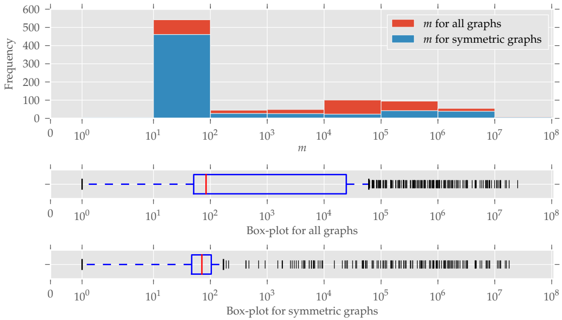
Figure 2. The histogram and box-plots for the number of edges m . The x-axis and the bin widths follow a log-scale. In every bin, a substantial amount of graphs contain symmetries. An explanation of why the graphs with 4 \leq \log_{10} m < 6 are relatively less-symmetric is given in the text. Nonetheless, symmetric graphs are present at all sizes.
