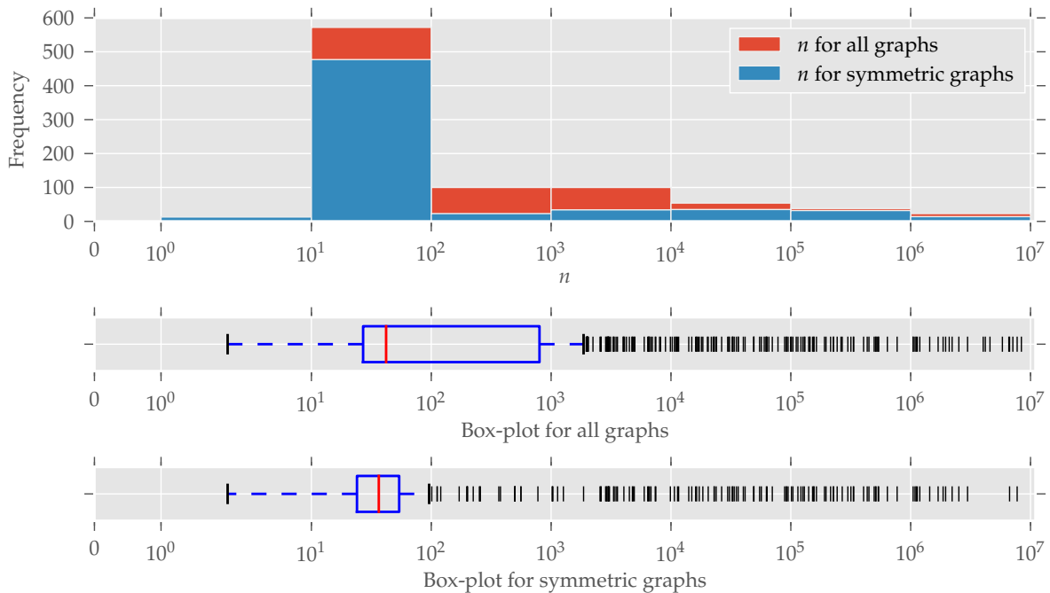
Figure A2. The histogram and box-plots for the number of nodes n . The x-axis and the bin widths follow a log-scale. Most graphs have between 10 and 100 nodes, and relatively fewer symmetries were found in medium-sized graphs, which coincides with the findings in Figure 2.
