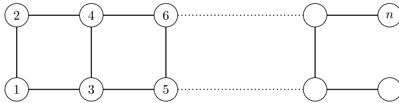
Figure A1. A graph of an even number of nodes n for which the normalized network redundancy does not capture the high degree of symmetry, as no node is fixed by the automorphism group. The example shows that the (normalized) redundancy does not distinguish between the questions how many redundancies exist ( r'_G \approx 0.5 means 50% of the nodes have a redundant counterpart) and how robust is an existing redundancy ( r'_G \approx 0.5 means 50% are structurally identical, therefore redundant, and the other 50% are not redundant).
