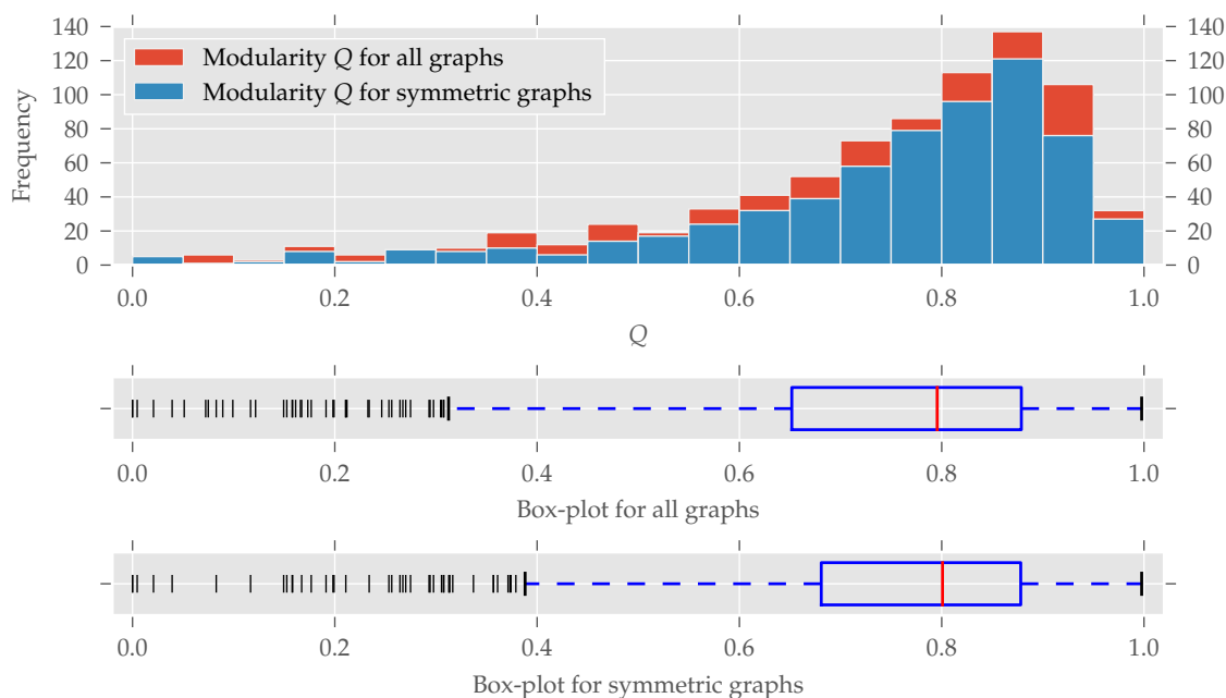
Figure A4. The histogram and box-plots for the modularity Q as in Figure 3.
