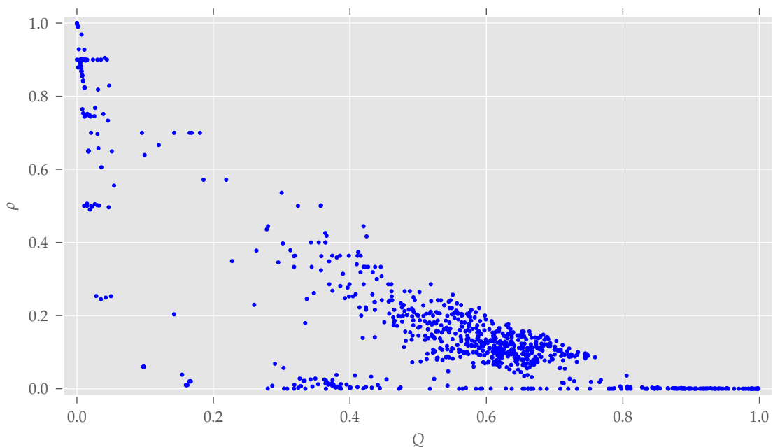
Figure A3. The density \rho := m/\binom{n}{2} of the graphs given their modularity Q . As stated in Section 4, modularity decreases with increasing density.
