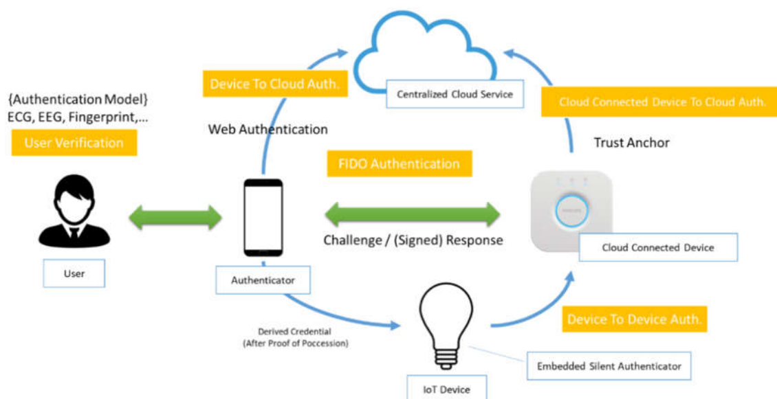
Figure 1. Emerging authentication technologies for IoT networks.
