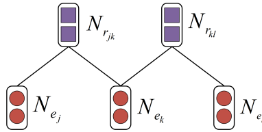
Figure 6. The symmetric relation between entity nodes and relation nodes in the entity-relation graph.
