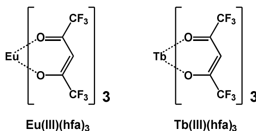
Figure 8. Optically inactive \text{Eu(III)(hfa)}_3 and \text{Tb(III)(hfa)}_3 .
