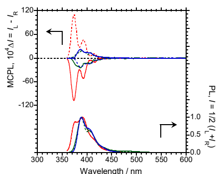
Figure 12. MCPL (upper panel) and PL (lower panel) spectra of Py (red lines), 1-PyOH (green lines), and 2-PyOH (blue lines) in N→S (solid lines) and S→N (dotted lines) magnetic directions under a 1.6 T magnetic field in CHCl 3 solution ( 1.0 \times 10^{-4} M).
