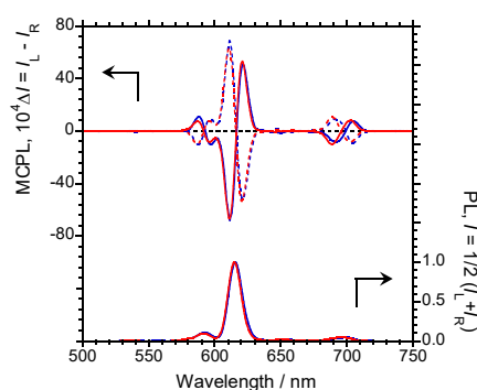
Figure 9. Magnetic circularly polarized luminescence (MCPL) (upper panel) and magnetic-field-induced unpolarized photoluminescence (PL) (lower panel) spectra of \text{Eu(III)(hfa)}_3 in N→S (solid lines) and S→N (dotted lines) configurations under a 1.6 T magnetic field in \text{CHCl}_3 (blue lines) and acetone (red lines) solutions ( 1.0 \times 10^{-3} M).
