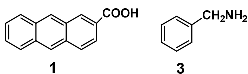
Figure 4. Achiral component molecules for circularly polarized luminescence (CPL).
