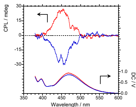
Figure 19. CPL (upper panel) and PL (lower panel) spectra of (R)-5 (red lines) and (S)-5 (blue lines) in \text{CHCl}_3 solution ( 1.0 \times 10^{-5} M).
