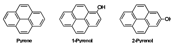
Figure 11. Achiral luminophores Py , 1-PyOH , and 2-PyOH .
