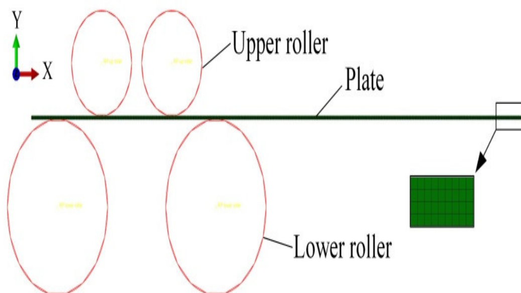
Figure 6. Numerical simulation model.
