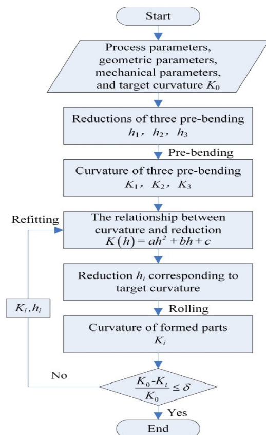
Figure 9. Flowchart of control strategy.
