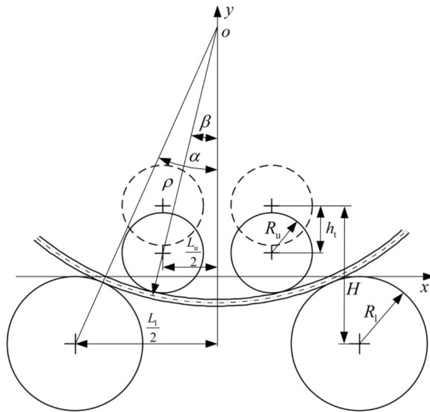
Figure 8. Geometric relationships in the roller bending process.
