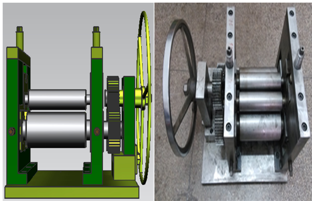
Figure 3. The SFRB device.
