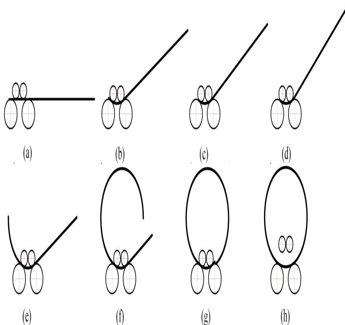
Figure 1. SFRB process: (a) feeding, (b) pre-bending, (c) reverse roll bending, (d) final bending, (e) positive roll bending, (f) positive roll bending, (g) bending completion, (h) unload and springback.
