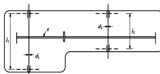
Figure 4. Weight Minimization of a Speed Reducer.
