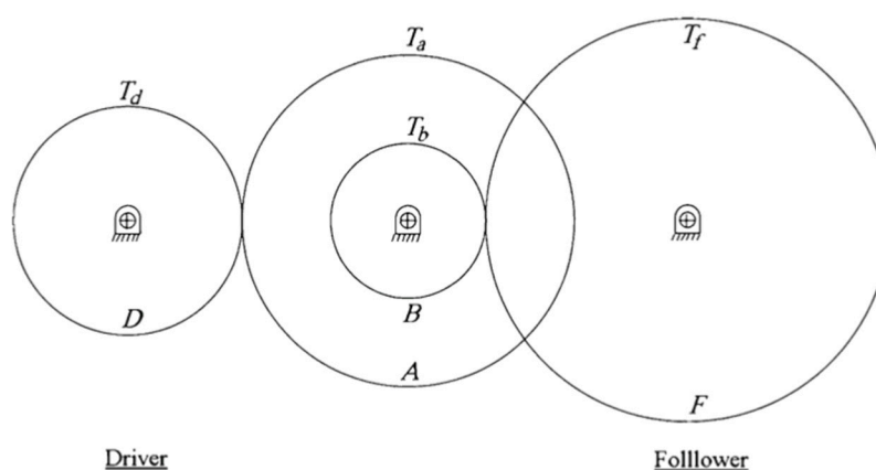
Figure 6. Gear train design Problem.
