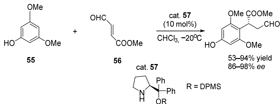
Scheme 20. Enantioselective alkylation of phloroglucinol derivatives.
