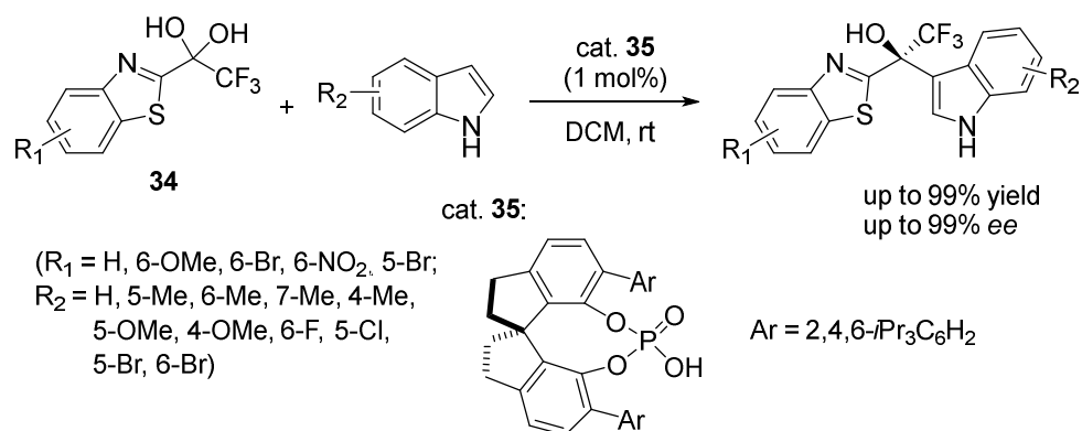
Scheme 13. Acid-catalyzed Friedel–Crafts alkylation of indoles.
