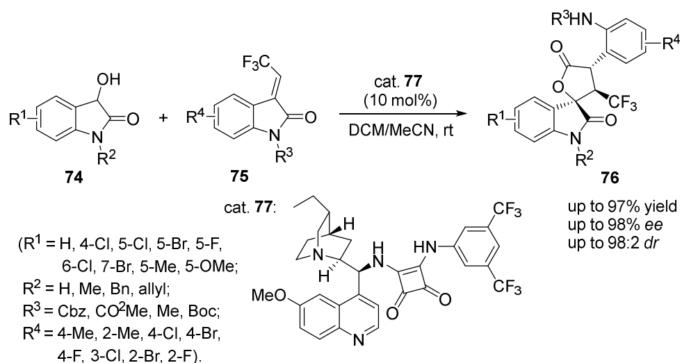
Scheme 29. Synthesis of spirooxindoles \gamma -lactones.
