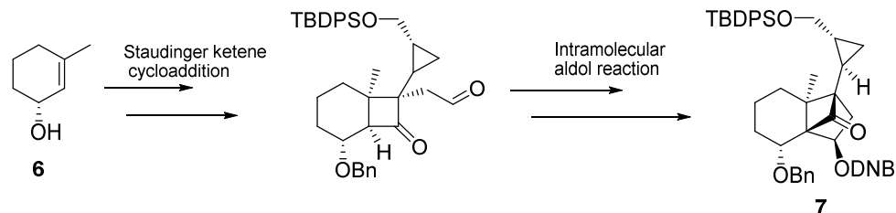
Scheme 2. Synthesis of solanoelepin A core starting from ( R )-seudenol.
