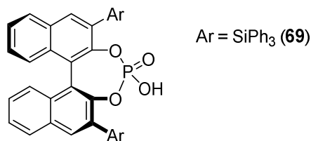
Scheme 27. Mannich reaction catalyzed by chiral phosphoric acid.
