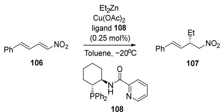
Scheme 35. Enantioselective addition of diethylzinc to nitrodiene.
