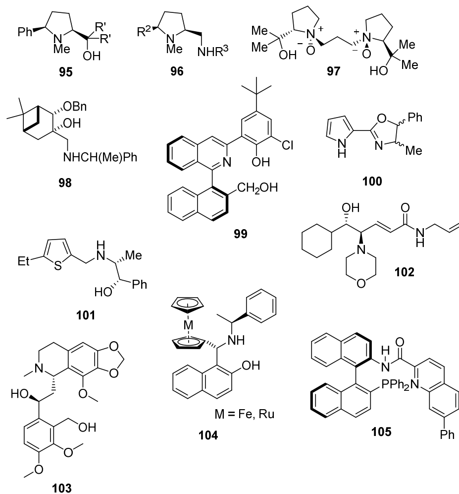
Figure 2. Catalysts for asymmetric diethylzinc addition to aldehydes.
