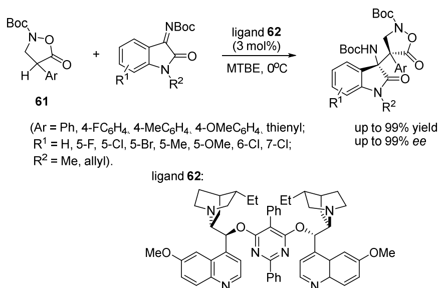
Scheme 23. Mannich reaction of isoxazolidin-5-ones with isatin-derived imines.
