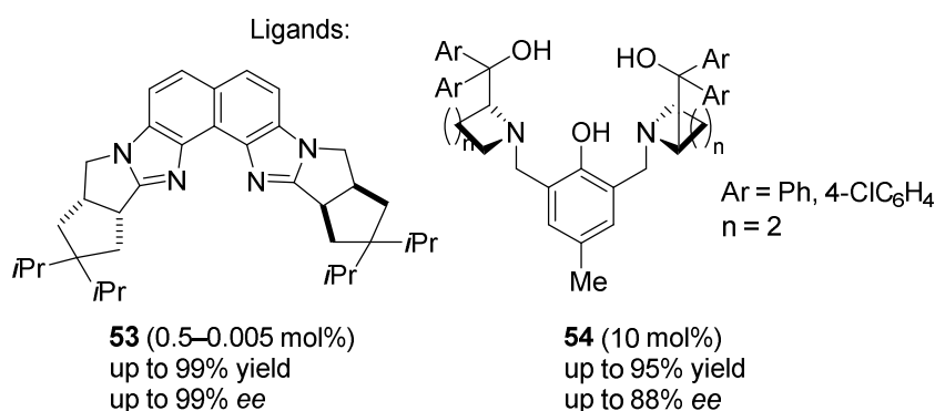
Scheme 19. Alkylation of indoles with trifluoromethyl pyruvates.
