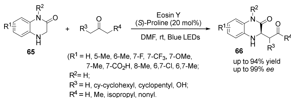
Scheme 25. Mannich reaction of dihydroquinoxalinones with ketones.
