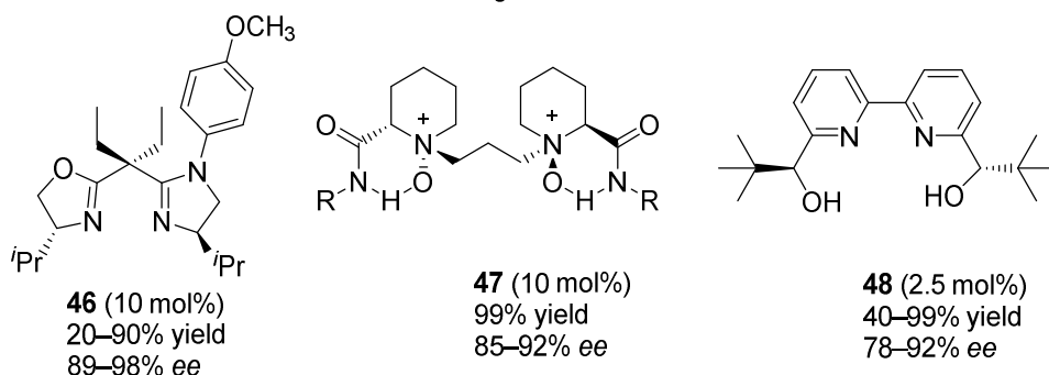
Scheme 17. Reaction of indole with enones.
