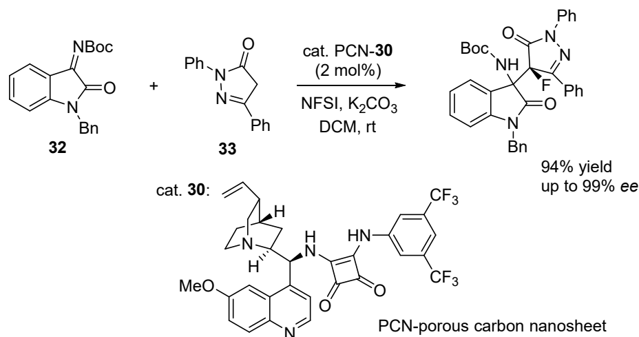
Scheme 12. Friedel–Crafts reaction of pyrazolone with isatin ketimine.
