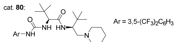
Scheme 30. Michael addition of pyrazol-5-ones to \alpha,\beta -unsaturated ketones.
