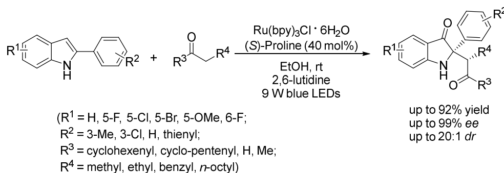
Scheme 26. Synthesis of C2-quaternary indolin-3-ones.
