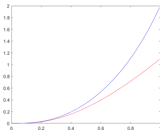
Figure 2. An example for the inequality (3) from Theorem 4 for the function \Psi(x) = x^4 and a = 0 , b = 1 , when \lambda = \frac{1}{2} .
