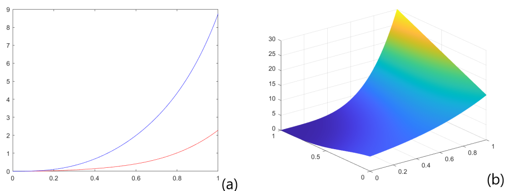
Figure 3. (a) An example for the inequality (3) from Theorem 4 for the function \Psi(x) = x^6 , a = 0 , b = 1 and \lambda = 1 ; (b) Graphic for the function {}_1 D_q^2 \Psi(x) from Example 3, considered as function of two variable x and q , when \Psi(x) = x^6 , a = 0 , b = 1 , and \lambda = 1 .
