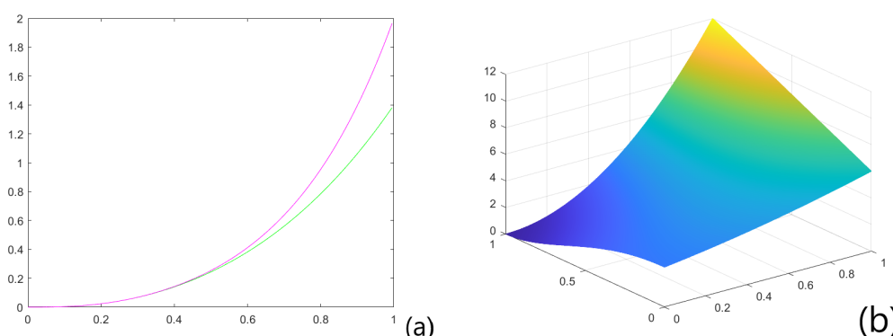
Figure 1. (a) An example for the inequality (3) from Theorem 4 for the function \Psi(x) = x^4 and a = 0 , b = 1 , when \lambda = 1 ; (b) Graphic for the functions {}^1D_q^2\Psi(x) , considered as function of two variables x and q , from Example 1 when \Psi(x) = x^4 , a = 0 , b = 1 , and \lambda = 1 .
