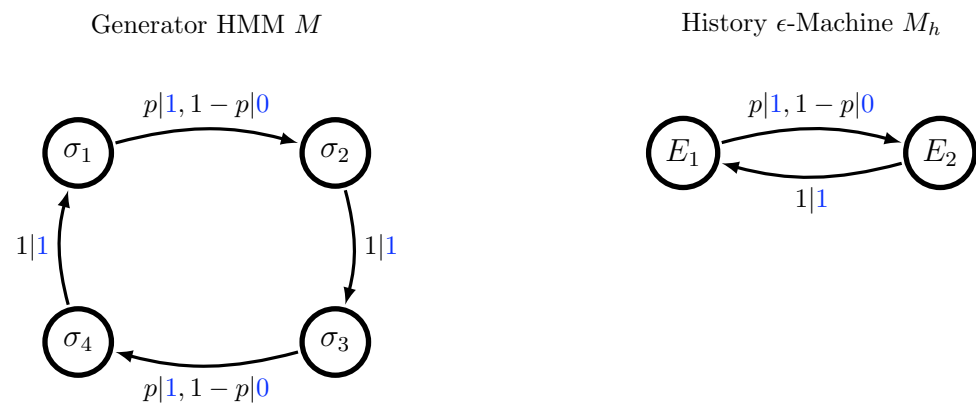
Figure 4. A nonminimal generating HMM M for the Noisy Period-2 (NP2) Process (left), and the associated history \epsilon -machine M_h for this process (right). p \in (0, 1) is a parameter.
