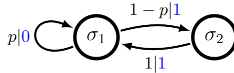
Figure 1. A hidden Markov model (the \epsilon -machine) for the Even Process. The HMM has two internal states S = \{\sigma_1, \sigma_2\} , a two-symbol alphabet \mathcal{X} = \{0, 1\} , and a single parameter p \in (0, 1) that controls the transition probabilities.
