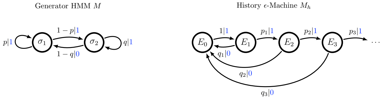
Figure 5. The Simple Nonunifilar Source (SNS) M (left) and associated history \epsilon -machine M_h (right) for the process \mathcal{P} generated by M . In the history \epsilon -machine, q_n + p_n = 1 for each n \in \mathbb{N} , and (q_n)_{n \in \mathbb{N}} is an increasing sequence defined by the following: q_n = (1 - q) \cdot \left( (1 - p) \sum_{m=0}^{n-1} p^m q^{n-1-m} \right) / \left( p^n + (1 - p) \sum_{m=0}^{n-1} p^m q^{n-1-m} \right) .
