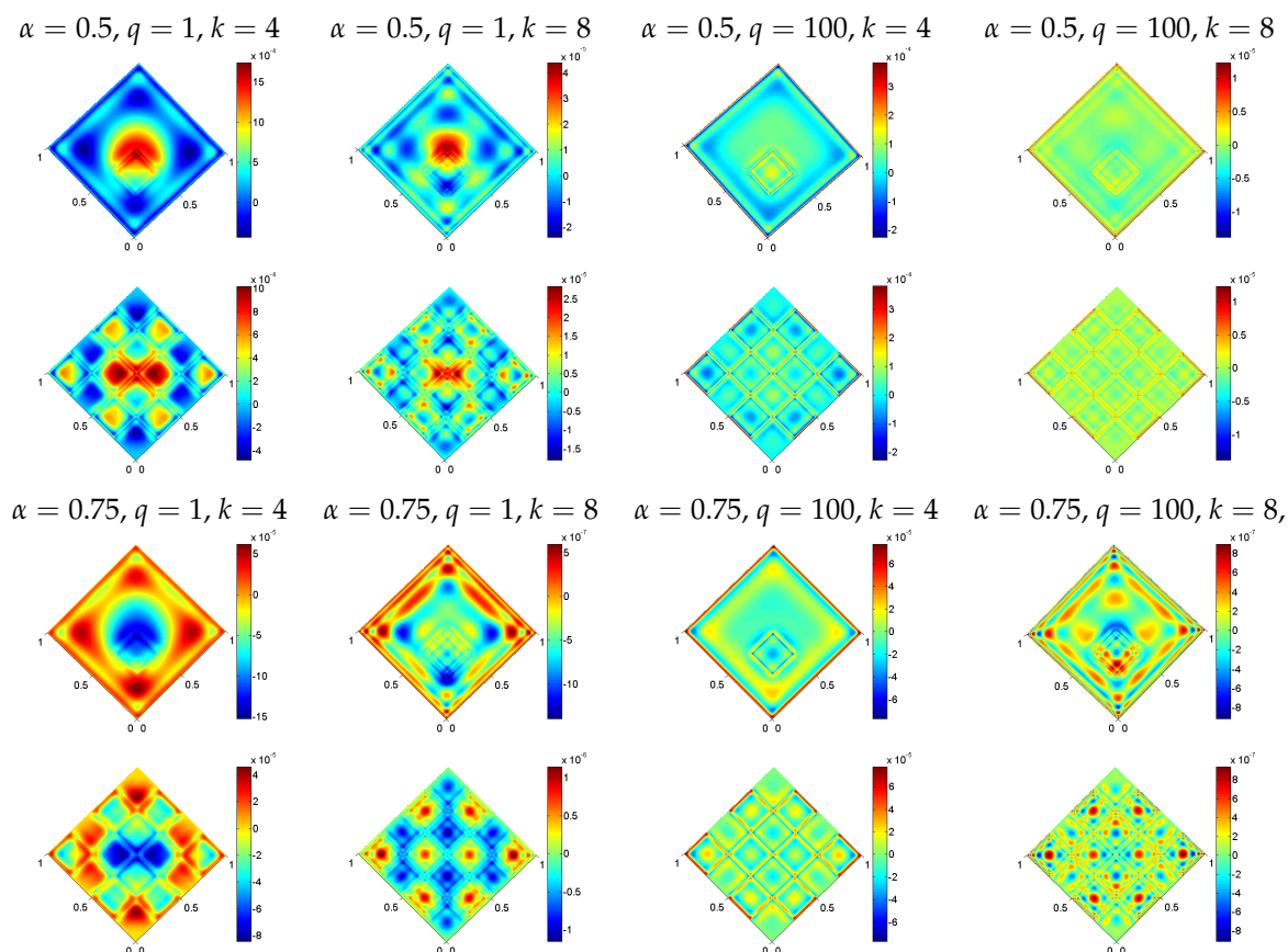
Figure 2. Numerical examples: Plots of the difference function u_k^{(2)} - u_k^{(1)} for the considered choices of \alpha, q, k . In each group, for \alpha \in \{0.5, 0.75\} , the first row of plots corresponds to f_1 and the second to f_2 .
