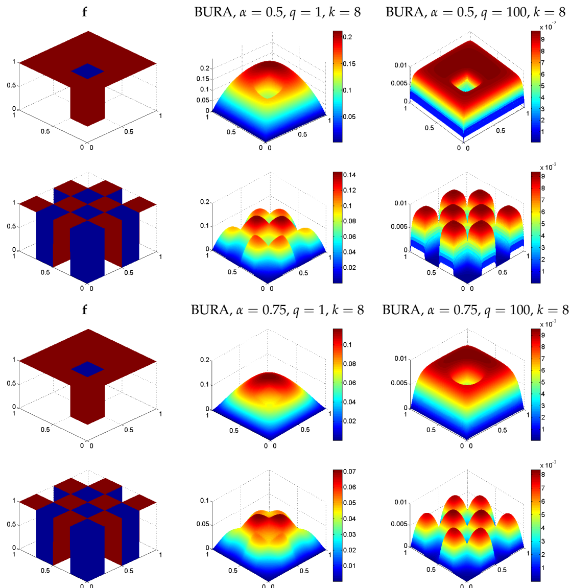
Figure 1. Numerical examples: The two choices for the right-hand side of (5) and their corresponding BURA solutions \mathbf{u}_g^{(2)} , with respect to the indicated parameters \alpha, q on [h, 1 - h] \times [h, 1 - h] , h = 2^{-10} .
