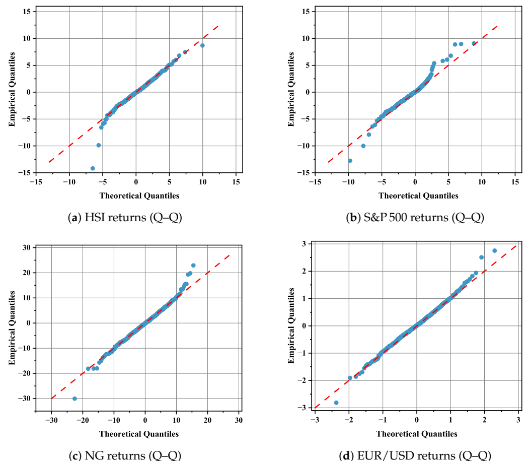
Figure 2. Q–Q plots comparing empirical return quantiles with the corresponding theoretical quantiles of the fitted SKTE distributions for four assets: (a) HSI, (b) S&P 500, (c) NG, and (d) EUR/USD. In each plot, the dots represent the empirical quantiles, and the dashed line represents the 45-degree reference line.
