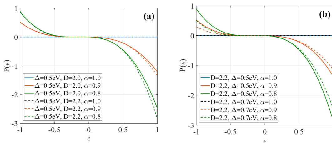
Figure 3. Particle-density asymmetry in doped BLG. Panel (a) shows the effects of \alpha and D at fixed interlayer coupling. In the pristine case ( \alpha = 1 , D = 2 ), the electronic occupation is symmetric between layers and P = 0 over the full energy range. Doped systems ( \alpha = 0.9, 0.8 ; D = 2, 2.2 ) exhibit a finite polarization, indicating preferential localization of electronic states in the doped layer. Panel (b) shows, for an inhomogeneous system ( D = 2.2 ), the competition between interlayer coupling and doping: increasing the interlayer hopping reduces the magnitude of P , restoring layer symmetry. Both figures were constructed using: \hbar = 6.58 \times 10^{-16} [eV · s]; v_F = 10^6 [m/s]; a = 2.46 \times 10^{-10} [m]; and L = 10a [m].
