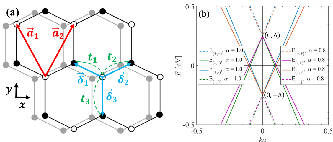
Figure 1. (a) Schematic of the bilayer graphene honeycomb lattice showing the primitive vectors \vec{a}_1 and \vec{a}_2 , the lattice vectors \vec{\delta}_1 , \vec{\delta}_2 , and \vec{\delta}_3 , and the hopping parameters t_1 , t_2 , and t_3 . The gray layer represents pristine graphene composed of carbon atoms, while the layer with white and black atoms corresponds to the doped graphene sheet with 50% carbon and 50% dopant atoms. (b) Energy band spectra of bilayer graphene obtained from Equation (2), where all branches are symmetric with respect to E = 0 . Here we contrast the pristine BLG case ( \alpha = 1 ) with the doped case ( \alpha = 0.8 ), showing the inner branches with solid lines and the outer branches with dashed lines.
