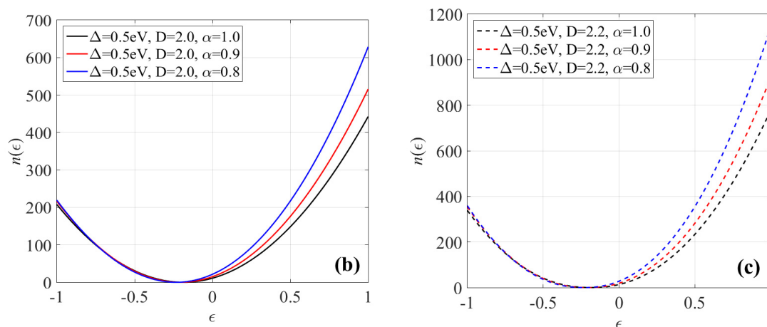
Figure 2. Cumulative number of states n(\varepsilon) in the interval -\tilde{\Delta} < \varepsilon < \tilde{\Delta} . Panel (a) shows pristine BLG ( \alpha = 1 ), illustrating the transition from a symmetric profile at \tilde{\Delta} = 0 to an asymmetric one at finite \tilde{\Delta} (using \Delta = 0.5 eV), for D = 2 and D = 2.2 . Panels (b,c) present doped BLG, comparing \alpha = 1 with \alpha = 0.9 and \alpha = 0.8 at finite \tilde{\Delta} (with \Delta = 0.5 eV), for D = 2 and D = 2.2 , respectively, highlighting the enhancement and asymmetry of \rho(\varepsilon) induced by doping and effective fractional dimensionality. All figures were constructed using: \hbar = 6.58 \times 10^{-16} [eV · s]; v_F = 10^6 [m/s]; \Delta = 0.5 [eV]; a = 2.46 \times 10^{-10} [m]; and L = 10a [m].
