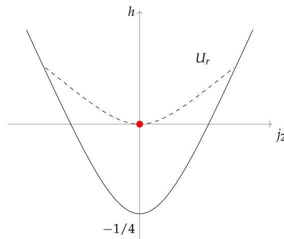
Figure 1. The set U_r of regular values in the momentum map.
