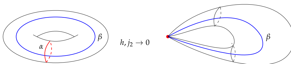
Figure 3. The singular fiber (pinched torus) at the focus–focus point.
