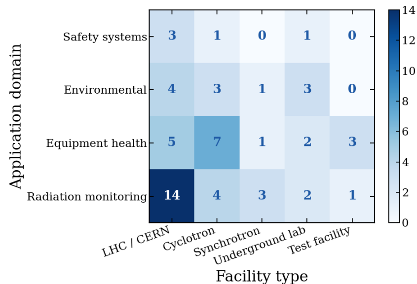
Figure 4. Heatmap showing the distribution of reviewed studies across application domains and facility types. Radiation monitoring applications dominate within LHC/CERN environments, while equipment-health studies are more broadly distributed across cyclotron and test-facility deployments.
