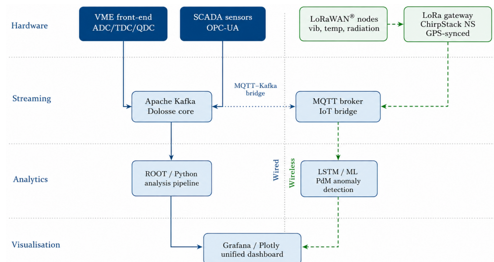
Figure 5. Integrated DAQ pipeline at NRF-iThemba LABS combining the Dolosse wired framework (solid lines), LoRaWAN ® auxiliary layer (dashed lines), and a unified Grafana frontend. Apache Kafka provides fault-tolerant streaming for wired physics signals; an MQTT-to-Kafka bridge integrates wireless IoT telemetry into the same pipeline, enabling unified ML-based predictive maintenance analytics.
