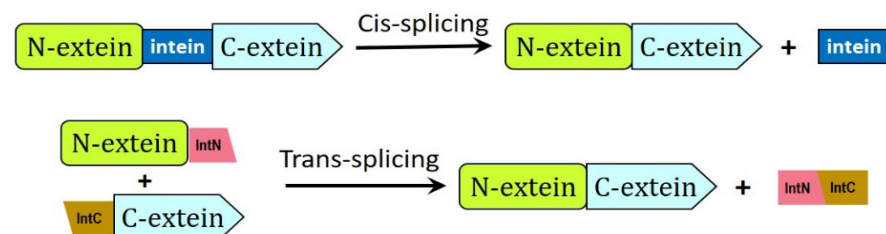
Figure 2. Cis- vs. trans-splicing via intein.
