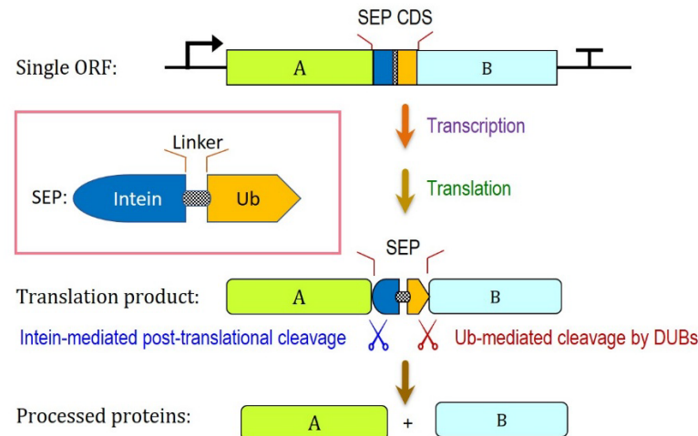
Figure 6. Mechanistic overview of intein-Ub SEP mediated protein coexpression. Note that the POIs preserve their native termini after cleavage from the polyprotein precursor. A & B: target proteins coexpressed.
