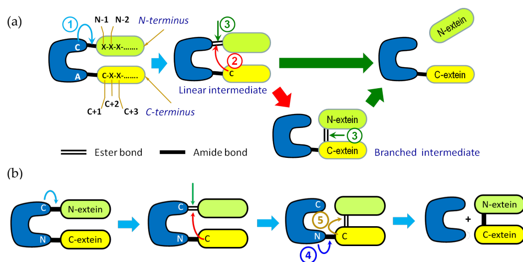
Figure 3. (a) N-terminal autocleavage process of an intein variant with a C-terminal Asn → Ala mutation. ① The nucleophilic thiol of the intein's N-terminal cysteine attacks the amide bond joining the N-extein to the intein, driving an N → S acyl shift that yields the linear intermediate. ② The N-extein is then relayed to the nucleophilic side chain of the C + 1 cysteine, forming a branched intermediate. ③ Hydrolysis of the unstable ester bond in the linear or branched intermediate, accelerated by mutating the flanking N- and/or C-extein residues, releases the cleaved N-extein. (b) Native intein splicing process. Following the same steps ① and ②, in step ④, the intein's C-terminal Asn cyclizes to a succinimide, cleaving the intein–C-extein amide bond and releasing the intein; ⑤ a spontaneous S → N acyl shift resolves the branched thioester into a native peptide bond, ligating the two exteins. A Cys at the +1 position is shown for illustration; Ser or Thr can serve the same role. Adapted from Amitai et al. [20].
