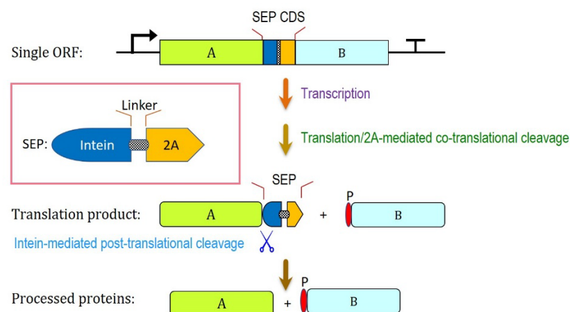
Figure 5. Mechanistic overview of multi-protein coexpression mediated by an intein-2A SEP. Intein provides precise and clean cleavage of POI-A, while 2A leaves a proline scar on the N-terminus of POI-B.
