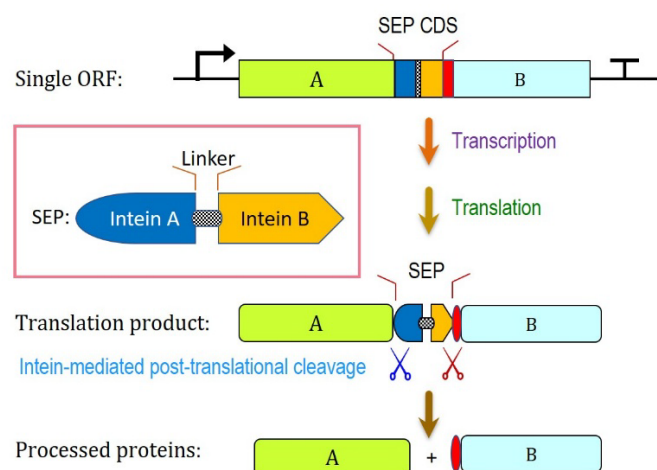
Figure 4. Mechanistic overview of dual-intein SEP mediated protein-coexpression. Note that the C + 1 residue of intein B (normally Cys, Ser, or Thr) becomes covalently appended to the N-terminus of POI-B after cleavage from the polypeptide precursor (indicated by the red oval). A & B: target proteins coexpressed.
