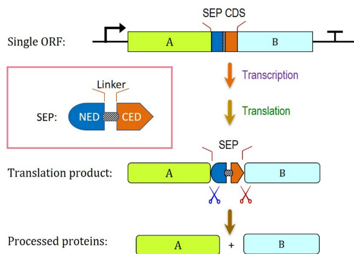
Figure 1. Working principle of SEP in coordinated multi-gene expression. A & B: target proteins coexpressed; CDS: coding sequence.
