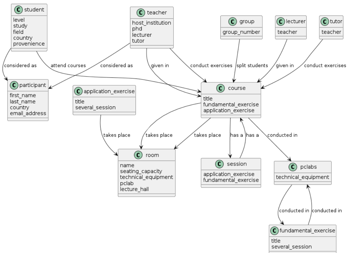
Figure 9. Class diagram generated for Text 2.
