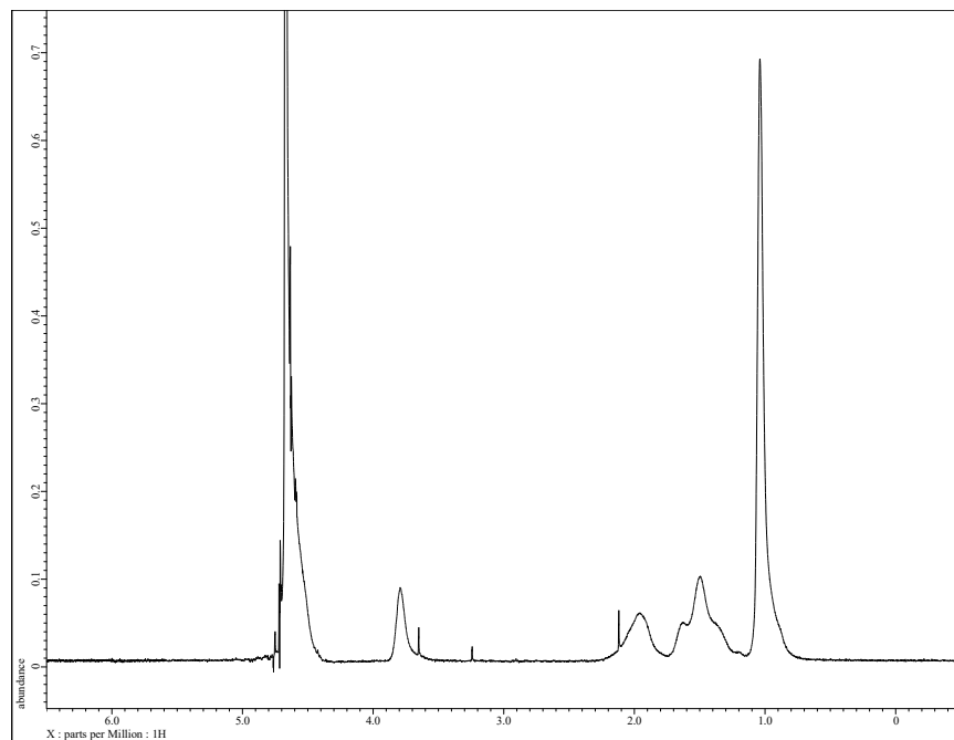
Poly(NIPAM- co -AM), Entry 2 in Table 2
