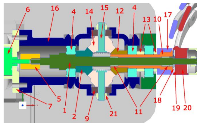
Figure 7. Contra-rotating gearbox section view.
