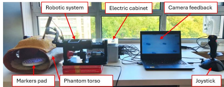
Figure 15. Experimental setup—robotic system and phantom torso.
