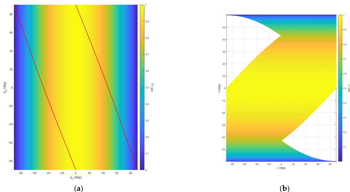
Figure 4. Conditioning and reachable orientation workspace of the spherical remote center-of-motion mechanism for \alpha_1 = 15^\circ : (a) absolute determinant of the orientation Jacobian J_3 over the actuated
