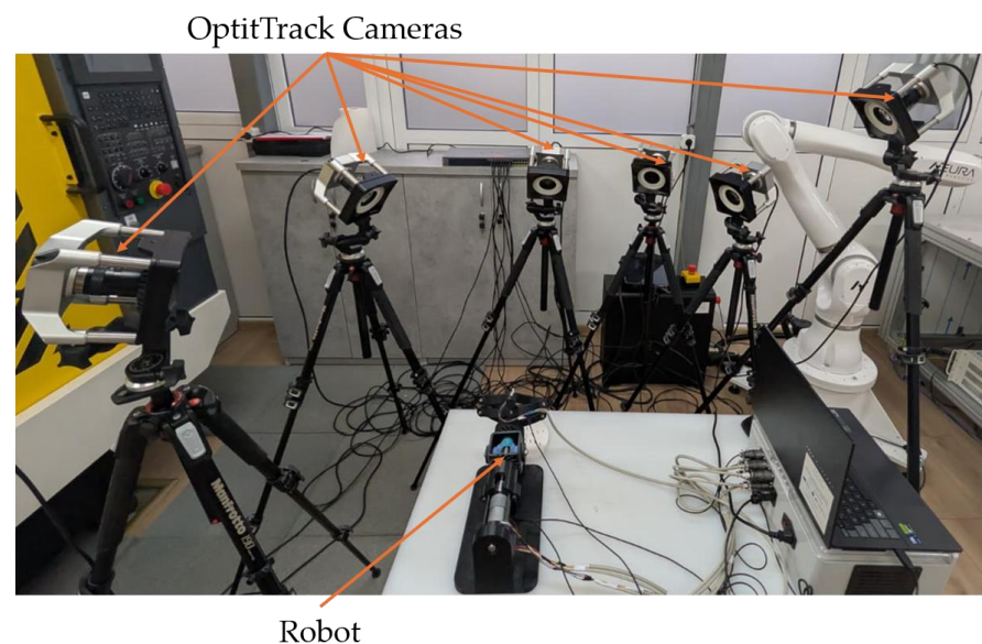
Figure 16. OptiTrack (NaturalPoint, Inc., Corvallis, OR, USA) measurement setup.
