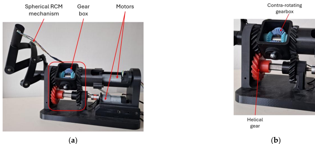
Figure 10. Final prototype and gearbox detail: (a) assembled robotic prototype; (b) detail of the contra-rotating gearbox.
