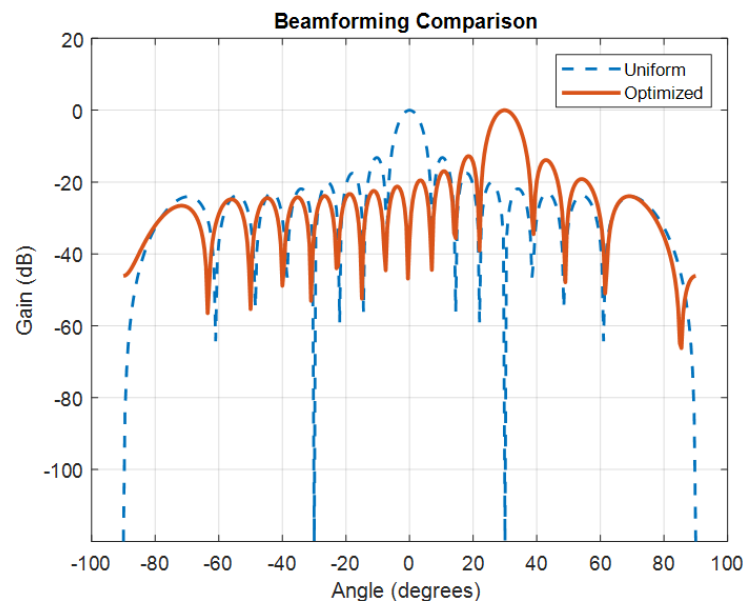
Figure 9. Beamforming results comparison.
