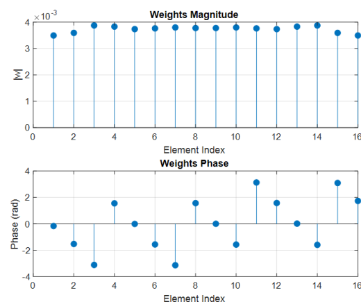
Figure 8. Phase distribution of the optimal weights used for beam steering.
