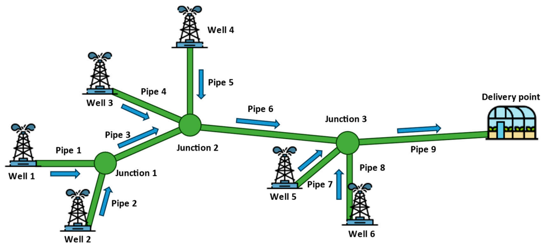
Figure 4. Schematic of the geothermal field.
