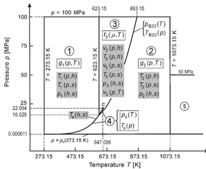
Figure 3. Regions and equations of IAPWS-IF97 [31].
