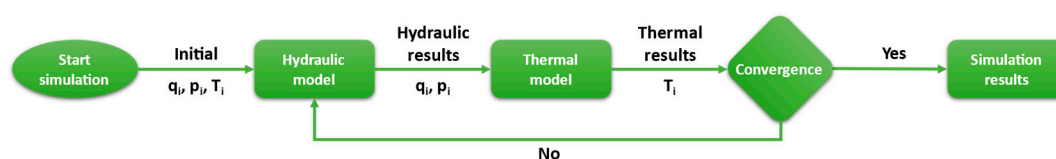
Figure 2. Flowchart of the circular solution of the coupled surface pipeline model. q : flowrate, p : pressure, and T : temperature.
