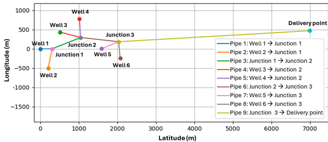
Figure 5. Scale map of the geothermal field.
