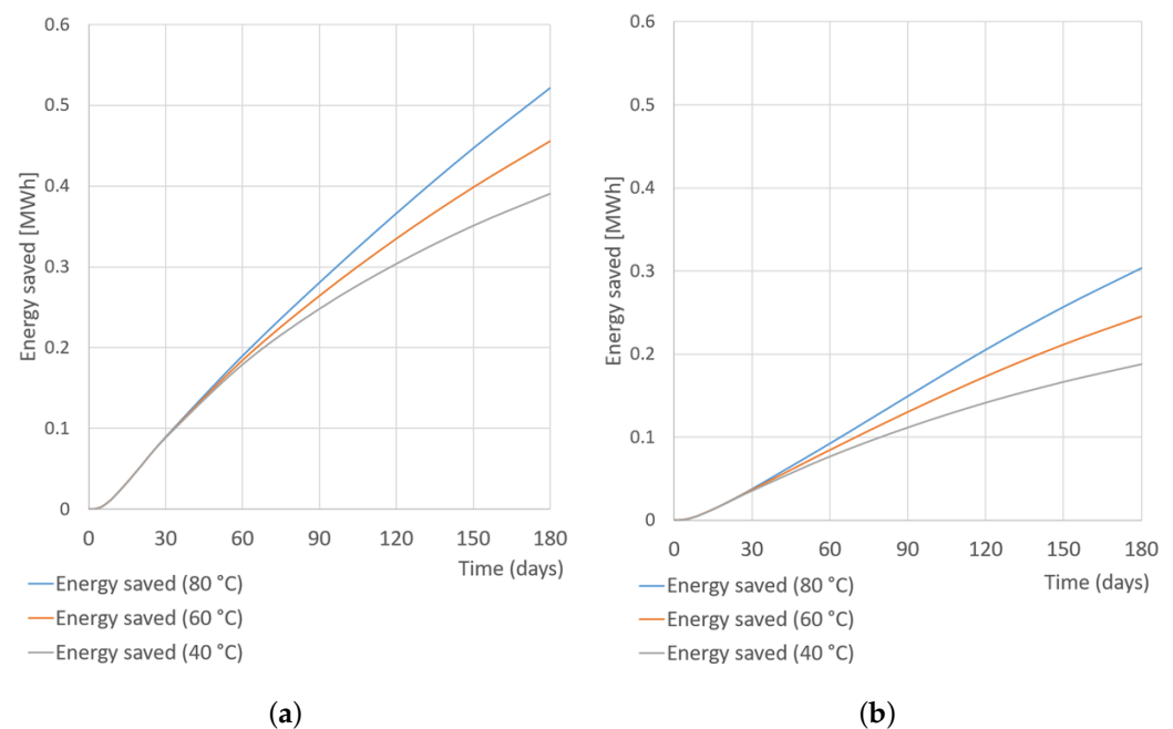
Figure 7. Stored energy gains over time for different surface insulation designs at heating setpoint temperatures of 40, 60, and 80 °C. (a) Effect of extending the surface insulation cover area (Configuration B relative to Configuration A) at an insulation thickness of 10 cm. (b) Effect of increasing the surface insulation layer thickness from 5 cm to 10 cm for Configuration A.
