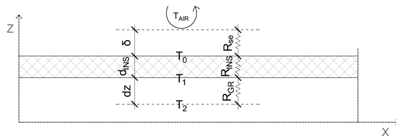
Figure 2. Schematic representation of the thermal resistance network used for the upper boundary condition at the surface insulation interface.
