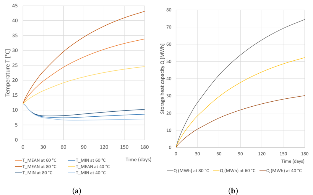
Figure 5. Transient evolution of average and minimum storage temperatures (a) and cumulative heat storage capacity (b) for varying BHE setpoint temperatures ( 40^\circ\text{C} , 60^\circ\text{C} and 80^\circ\text{C} ) with a surface insulation area of 9 \times 9 m and 10 cm insulation thickness.
