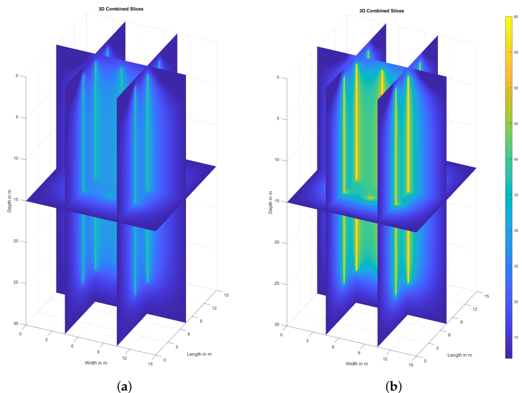
Figure 6. Three-dimensional temperature distributions after 180 days for heating setpoint temperatures of 40 °C (a) and 60 °C (b). Both cases assume a 9 \times 9 m surface insulation area with a thickness of 10 cm.
