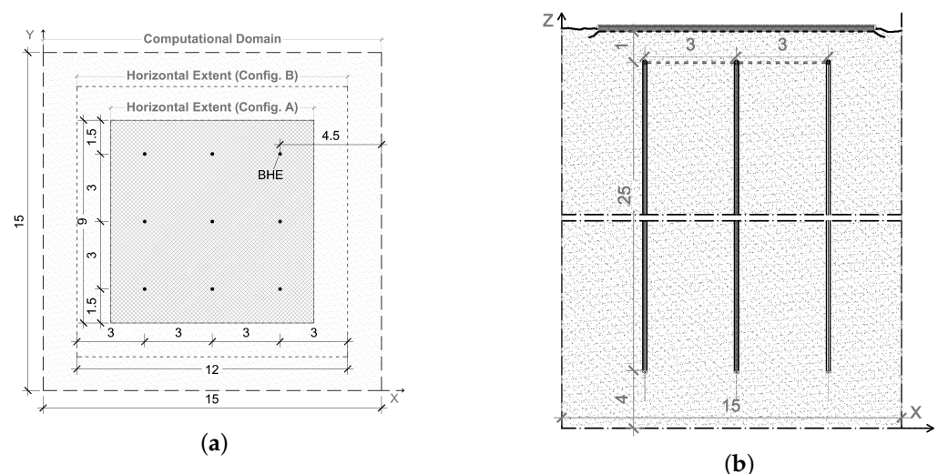
Figure 1. Top view (a) and vertical cross-section (b) of the BTES field.
