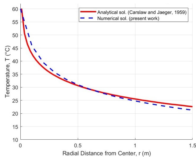
Figure 3. Model verification with an exact analytical solution [33] after 180 days.
