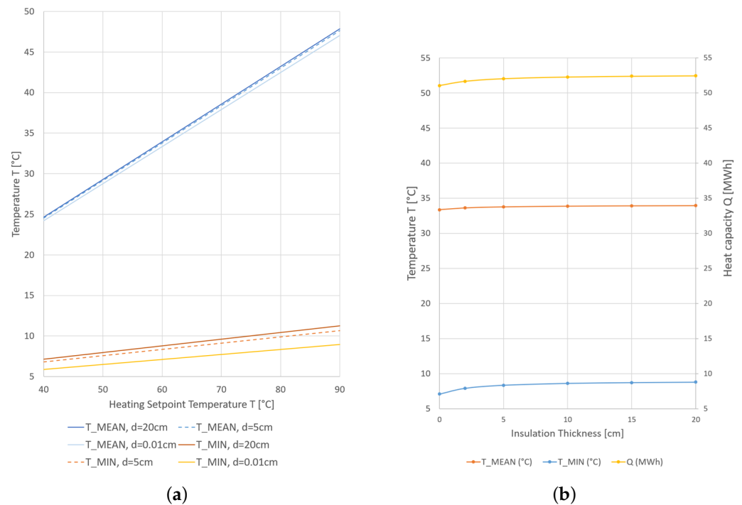
Figure 4. (a) Average and minimum temperatures as functions of heating setpoint temperature and insulation thickness (Configuration A scenario). (b) Average and minimum temperatures and total storage capacity for varying insulation thicknesses at a heating setpoint temperature of 60 °C. (Configuration A scenario).
