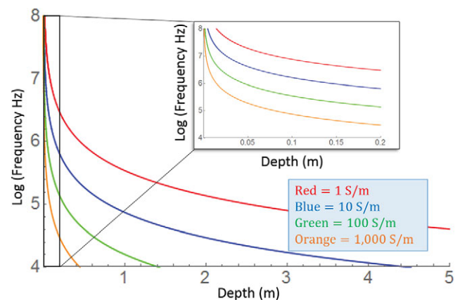
Figure 8. Two-dimensional plots showing electromagnetic wave decay as a function of frequency and material depth. Lines show the frequencies and depths at which a wave is 50% attenuated for a given conductivity. The larger the conductivity, the more frequencies are attenuated at a given depth. In conductive material, the attenuation of high frequency components creates a low-pass filter that accounts for the temporal delay seen in simulations. Inset shows the boxed magnified.
