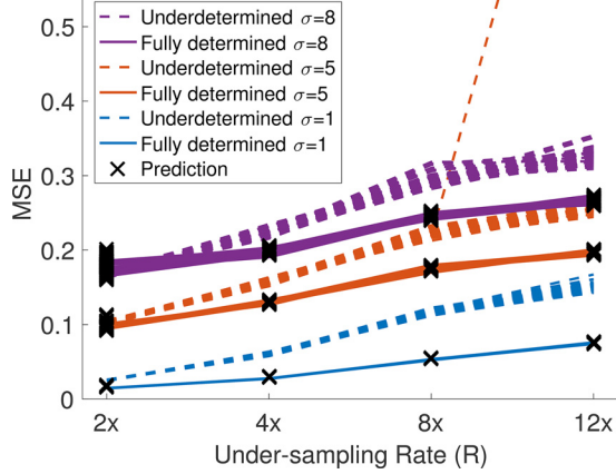
Figure 6. Results of our experiment to compare fully determined and underdetermined reconstructions with the same total measurement time across four different undersampling rates (2×, 4×, 8×, 12×) for three different noise levels (added noise standard deviations 1.0, 5.0, 8.0). Mean squared error (MSE) values are plotted for each of the 100 repetitions of the same experiment. Note that for the 2× undersampling rate, the fully determined and underdetermined reconstructions have essentially the same MSE. As the undersampling rate increases, the underdetermined system produces an increasingly worse MSE than the fully determined system. Note that one of the 100 underdetermined reconstructions at \sigma = 5 and R = 12\times failed to converge. This outlier is consistent with compressed sensing theory and practice where the reconstruction may fail to converge at higher undersampling rates.
