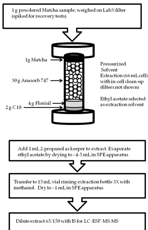
Figure 1. Sample preparation method for conazole fungicide analysis.
