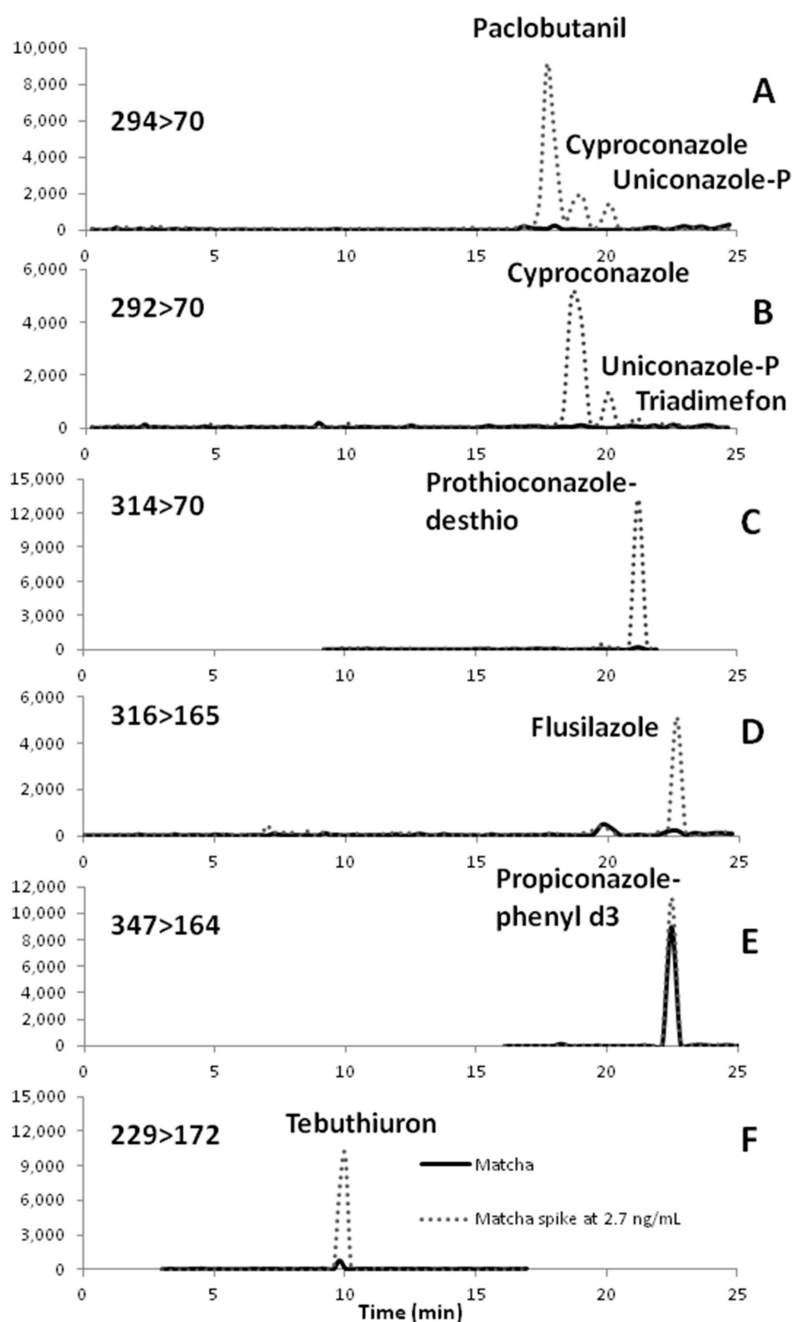
Figure 2. Selected Reaction Monitoring (SRM) Chromatograms of Matcha and Matcha Spiked with Standard Solution. Sample size of 1 g of Matcha with pre-concentrated of pressurized solvent extraction extract to a volume of 1 mL with extract diluted by factor of 0.43 with methanol. Sample extract is spiked at level of 2.67 ng/mL of standard mixture of conazole fungicides and structurally similar pesticides. Internal standard (propiconazole-phenyl d 3 ) added to sample at concentration of 50 ng/mL. SRM Chromatograms: A, SRM 294>70; B, SRM 292>70; C, SRM 314>70; D, SRM 316>165; E, SRM 347>164; F, SRM 229>72. See Table 1 for retention times of analytes.
