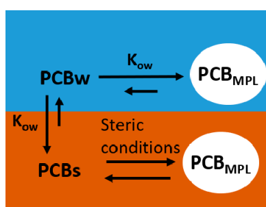
Figure S2. Schematic diagram on sediment, water, and MPLs partitioning for PCBs.
