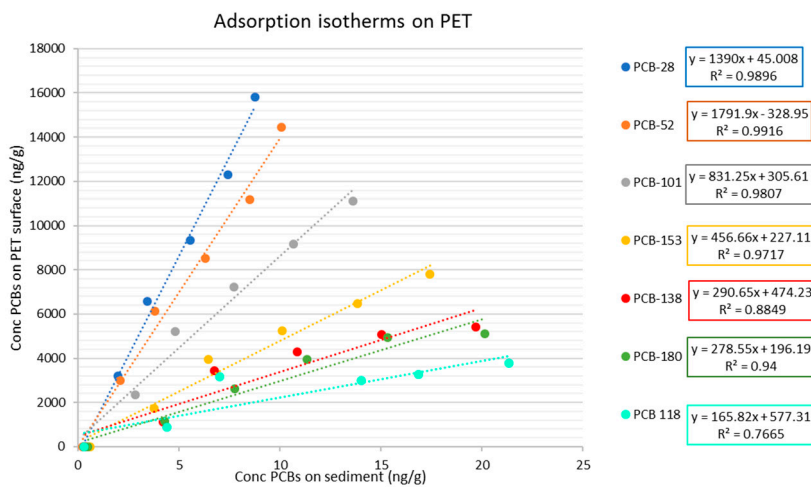
Figure S3. Individual adsorption isotherms of marker PCBs on (A) PS, (B) PE and (C) PET.
