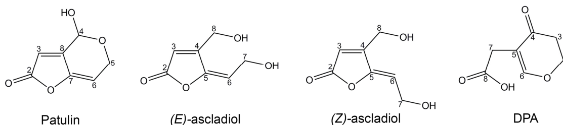
Figure 1. Chemical structures of patulin and its breakdown products ( E ) and ( Z ) ascladiol, and desoxypatulinic acid (DPA).
