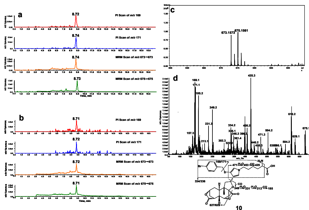
Figure 2. (a) Mass spectrometric profiles obtained from a four-channel scanning system analysis of mouse liver microsomal incubations containing DIOB, NADPH, Lys, and BBM; (b) Mass spectrometric profiles obtained from the four-channel scanning system analysis of mouse liver microsomal incubations containing DIOB, NADPH, and BBM, followed by exhaustive proteolytic digestion; (c) High resolution mass spectrum; (d) MS/MS spectrum of pyrrole 10 .
