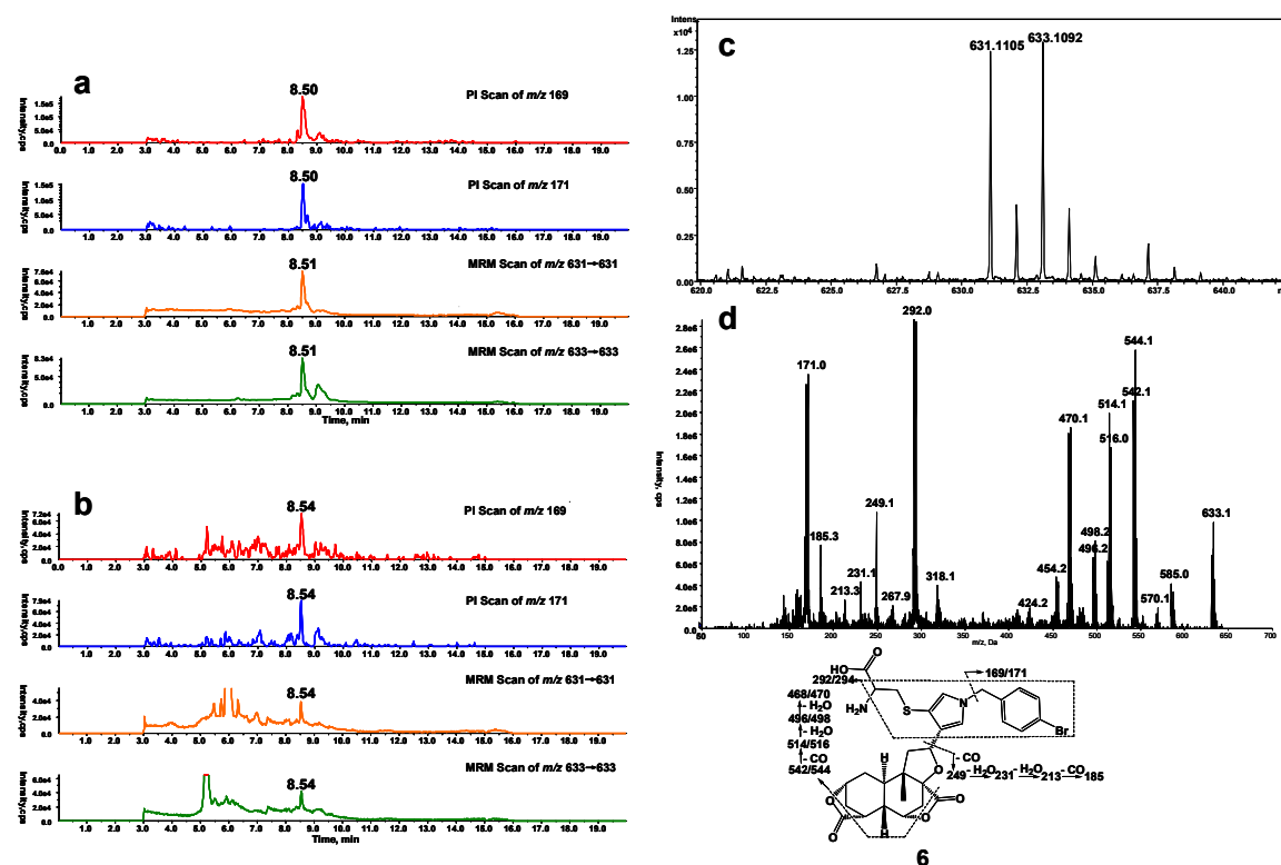
Figure 1. (a) Mass spectrometric profiles obtained from a four-channel scanning system analysis of mouse liver microsomal incubations containing DIOB, NADPH, Cys, and BBA; (b) Mass spectrometric profiles obtained from the four-channel scanning system analysis of mouse liver microsomal incubations containing DIOB, NADPH, and BBA, followed by exhaustive proteolytic digestion; (c) High resolution mass spectrum; (d) MS/MS spectrum of pyrrole 6 .
