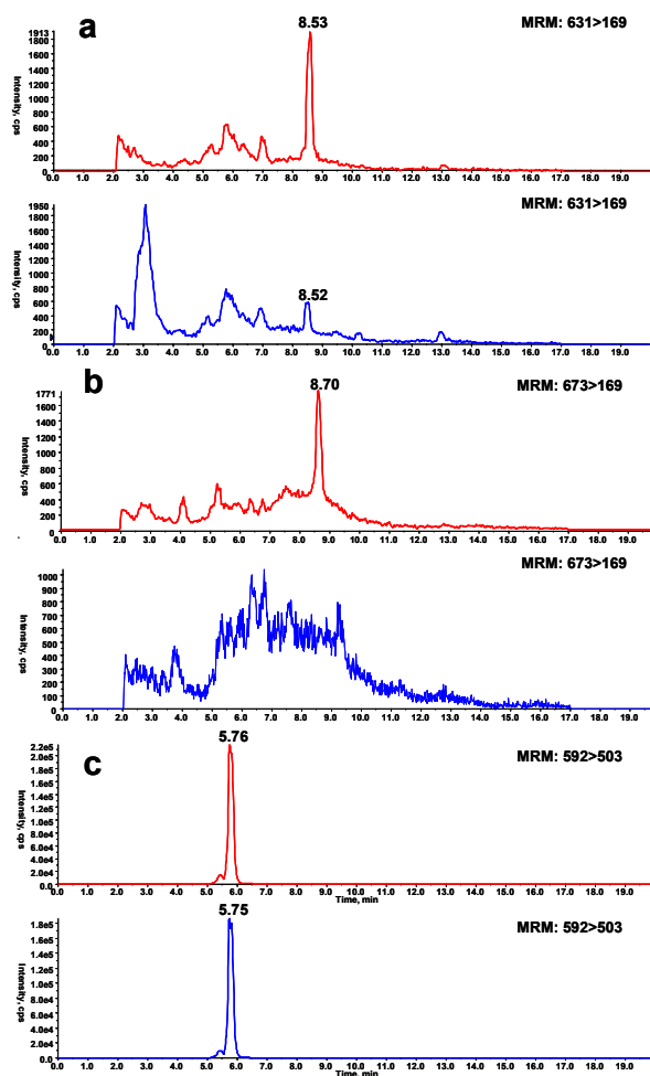
Figure 4. DIOB was incubated with mouse liver microsomes in the presence of NADPH, followed by reaction with BBA before (red) or after (blue) dialysis and analysis by MRM scanning (ion transition m/z 631→169) (a), followed by reaction with BBM before (red) or after (blue) dialysis and analysis by MRM scanning (ion transition m/z 673→169) (b). (c) Similar incubations were performed with (blue) or without (red) dialysis before proteolytic digestion and analysis by MRM scanning (ion transition m/z 592→503).
