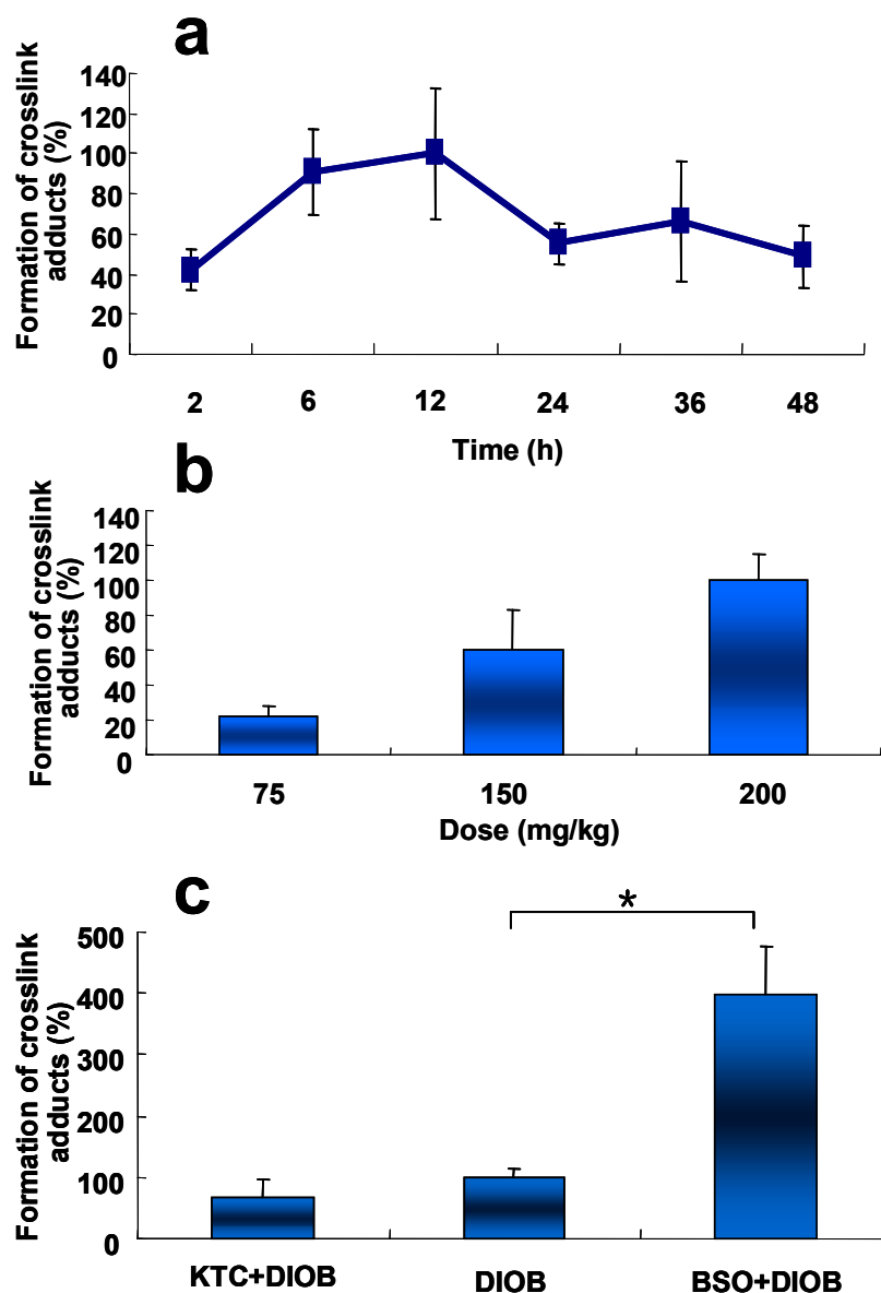
Figure 6. (a) Time-course changes in level of pyrrole 12 in mice treated with DIOB (i.p.) at 200 mg/kg −1 ( n = 3 ); (b) Dose-dependent changes in level of pyrrole 12 in mice given DIOB (i.p.) at various dosages ( n = 3 ); (c) Protective effect of KTC and synergistic effect of BSO on DIOB-induced hepatic protein modification. Mice were administered KTC (75 mg/kg/d, 2 days) + DIOB (200 mg/kg), DIOB (200 mg/kg) alone, or BSO (666 mg/kg) + DIOB (200 mg/kg) ( n = 3 ). * P < 0.05 were considered significantly different.
