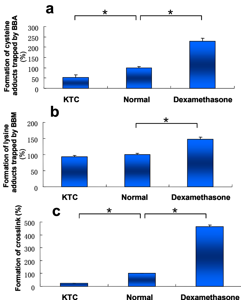
Figure 5. Levels of pyrrole 6 (a), pyrrole 10 (b), and pyrrole 12 (c) detected in microsomal incubations, containing DIOB, NADPH, and liver microsomes obtained from mice pretreated with KTC (75 mg/kg/d, 2 days), vehicle, or DEX (50 mg/kg/d, 5 days) ( n = 3 ). * P < 0.05 were considered significantly different.
