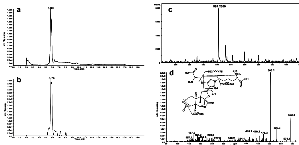
Figure 3. (a) Mass spectrometric profiles obtained from MRM scanning (ion transition m/z 592→503) analysis of mouse liver microsomal incubations containing DIOB, NADPH, Lys, and Cys; (b) Mass spectrometric profiles obtained from MRM scanning (ion transition m/z 592→503) analysis of mouse liver microsomal incubations containing DIOB and NADPH, followed by exhaustive proteolytic digestion; (c) High resolution mass spectrum; (d) MS/MS spectrum of pyrrole 12 .
