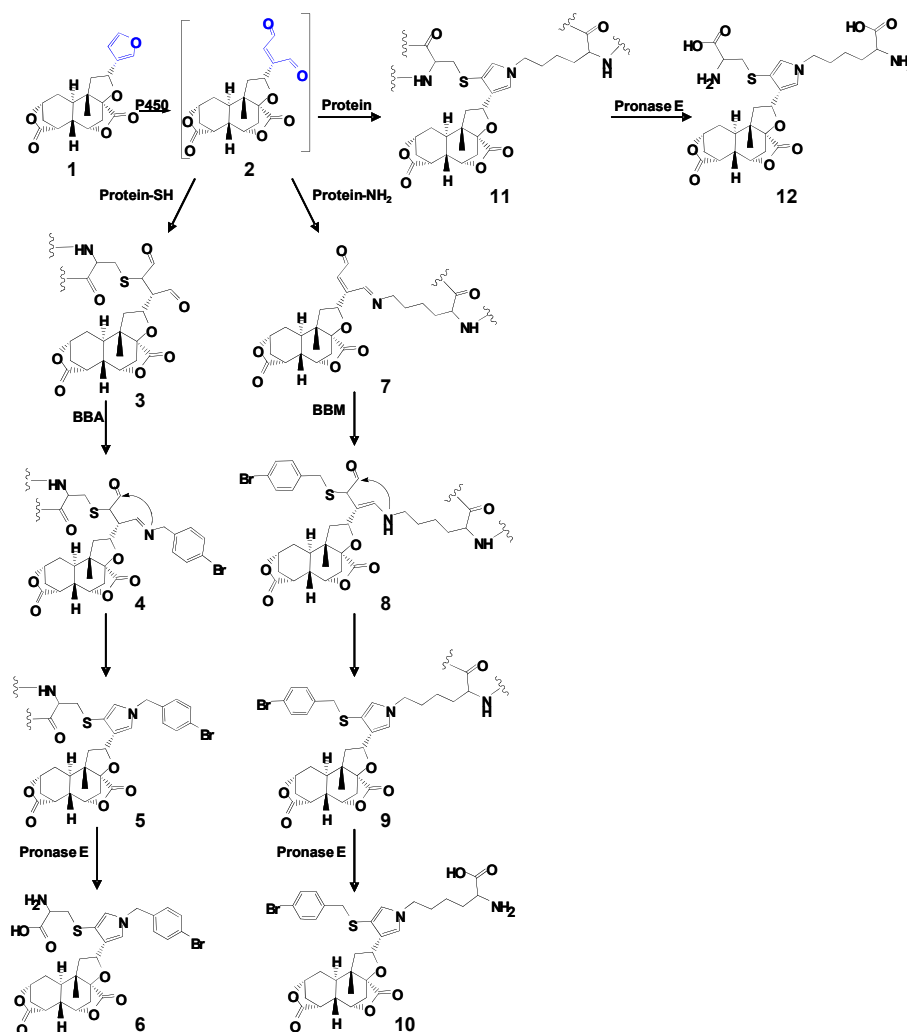
Scheme 1. Proposed pathways of protein/amino acid residue adduct formation as a result of DIOB bioactivation.
