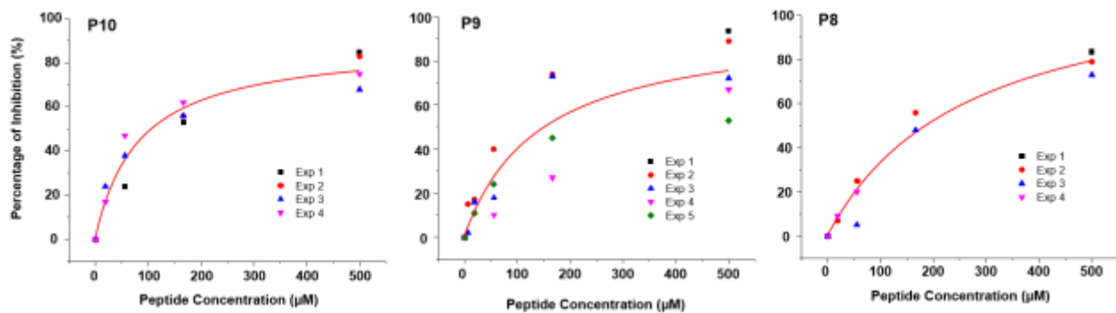
Figure S2. Inhibition of depurination activity of RTA on rat liver ribosomes by peptides P10, P9, and P8. The IC 50 values were determined as in Figure 6 and are shown in Table 2.
