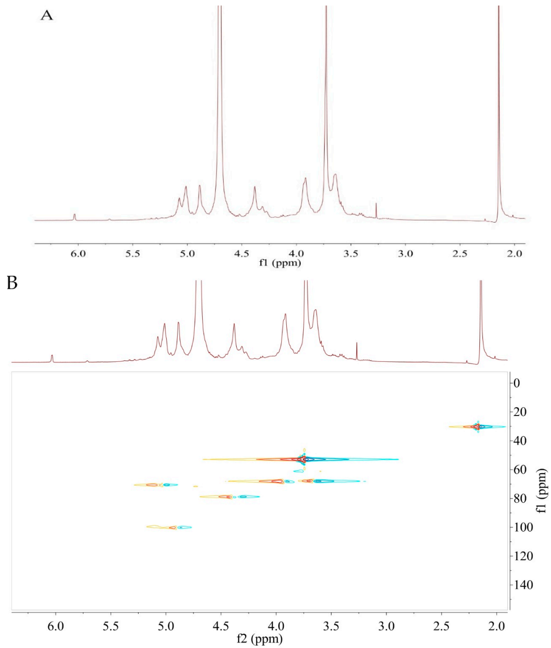
Figure S2. NMR spectra of ripe banana peel polysaccharides. (A) 1 H spectra; (B) HSQC Spectra.
