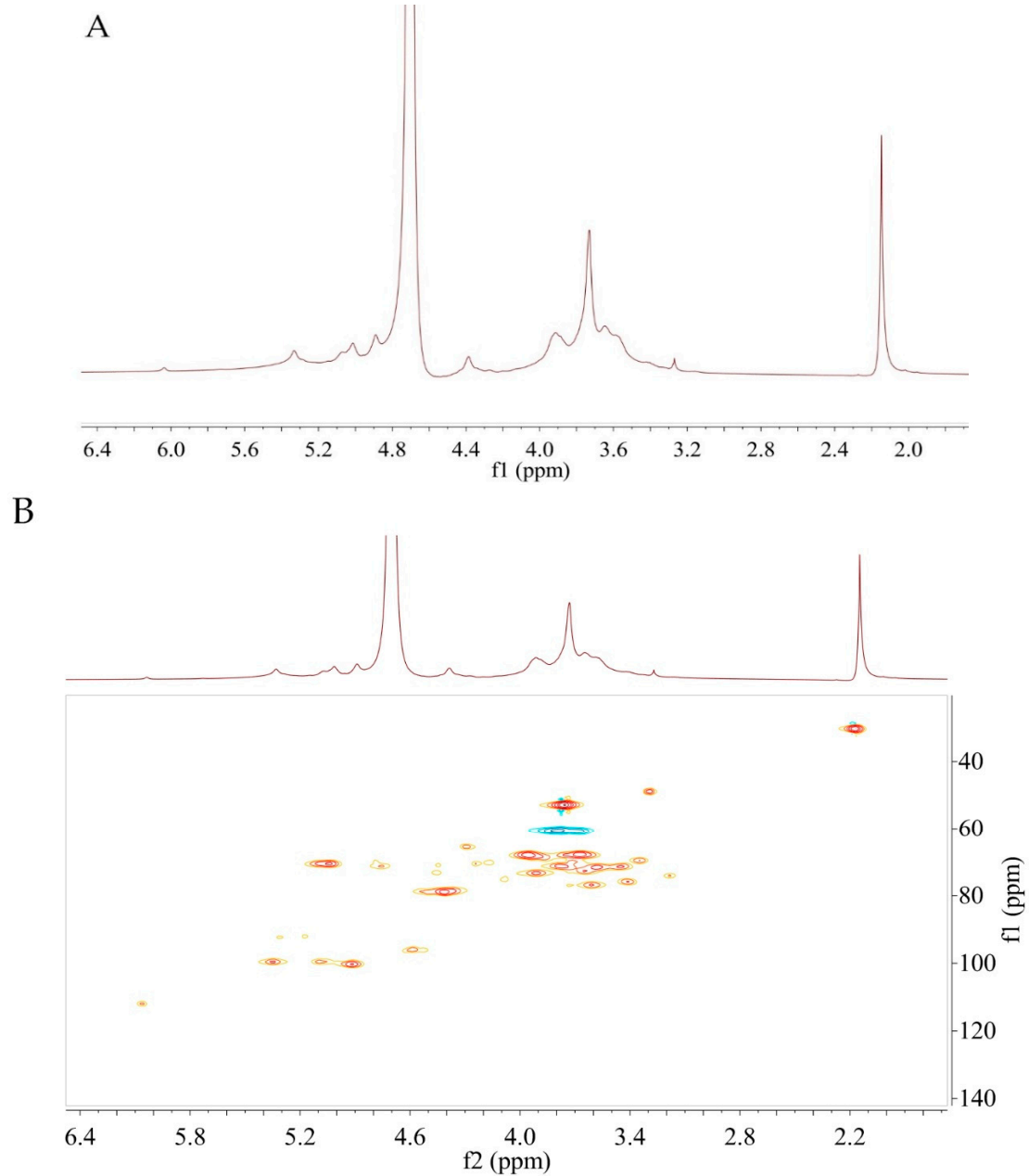
Figure S1. NMR spectra of unripe banana peel polysaccharides. (A) ^1\text{H} spectra; (B) HSQC Spectra.
