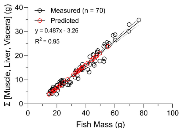
Figure 5. Combined sum of measured tissue masses ( \Sigma [muscle + liver + viscera]) (black) of all L. rhomboides sampled in this study as a function of total fish mass. Total body masses at the start of depuration were estimated using an exponential growth formula (see Methods) and were used to estimate the \Sigma [muscle + liver + viscera] (red) for each fish at experiment day 20 which entered the depuration phase ( n = 24 ). Dashed lines are 95% confidence intervals.
