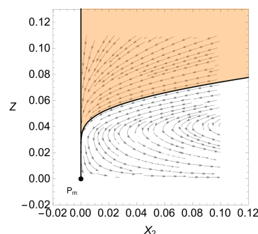
Figure A1. Nonhyperbolic fixed point P_m .
